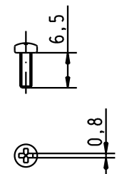
Flathead screws
