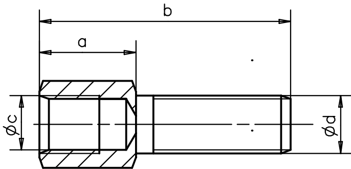
SCREW - LOCK UNC 4-40 / UNC 4-40
