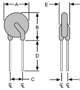
Figure 2 FBR550F ~ FBR900F Lead Size: 20AWG Φ 0.81 mm Diameter
