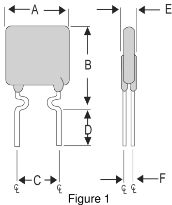
Figure 1 FRU 090-30F ~ FRU 250-30F Lead Size: 24AWG, Φ 0.51 mm Diameter
