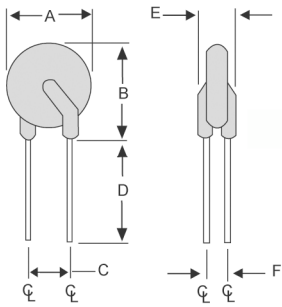
Figure 1 Lead Size: 24AWG Φ 0.51 mm Diameter
