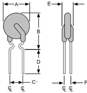
Figure 1 FRX 005-60F ~ FRX 090-60F Lead Size: 24AWG, Φ 0.51 mm Diameter
