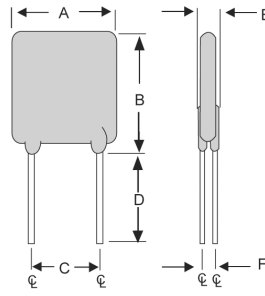
Figure 2 Lead Size: 20AWG Φ 0.81 mm Diameter
