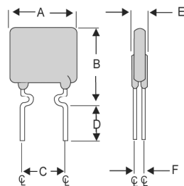
Figure 2 Lead Size :24AWG Φ0.51 mm Diameter
