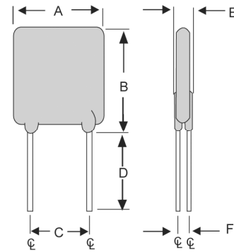
Figure 2 FRU 300-30F ~ FRU 900-30F Lead Size: 20AWG Φ 0.81 mm Diameter
