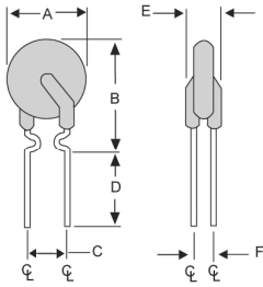
Figure 1 Lead Size :24AWG Φ0.51 mm Diameter
