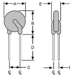
Figure 2 FRA110-120F ~ FRA375-120F Lead Size : 20AWG, Φ 0.81 mm Diameter
