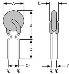
Figure 1 FRA010-120F ~ FRA090-120F Lead Size: 22AWG, Φ 0.65 mm Diameter
