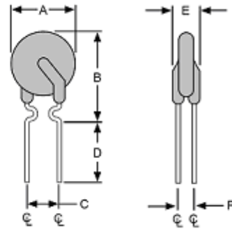
Figure 2 Lead Size: 24AWG Φ 0.51 mm Diameter
