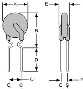
Figure 1 FBR100F ~ FBR350F Lead Size: 24AWG Φ 0.51 mm Diameter
