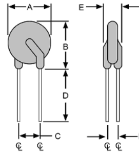
Figure 2 FRX 110-60F ~ FRX 375-60F Lead Size: 20AWG, Φ 0.81 mm Diameter
