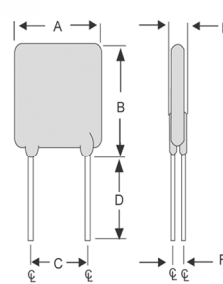
Figure 3 Lead Size: 20AWG Φ 0.81 mm Diameter
