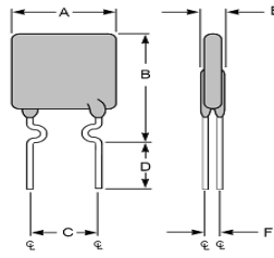
Figure 2 FRK110-60F Lead Size : 20AWG Φ 0.81 mm Diameter
