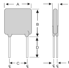
Figure 3 FRK135-60F~FRK500-60F Lead Size : 20AWG Φ 0.81 mm Diameter
