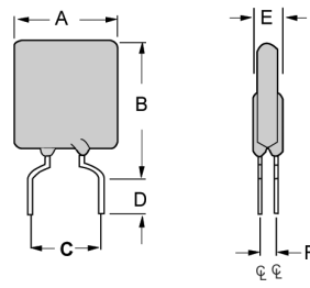
Figure 3 Lead Size : 20AWG Φ 0.81 mm Diameter
