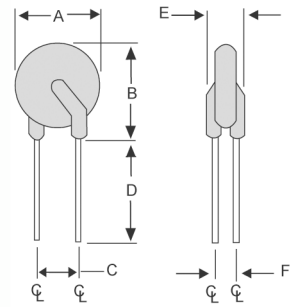
Figure 4 Lead Size: 20AWG Φ 0.81 mm Diameter
