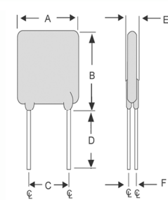
Figure 2 Lead Size: 22AWG Φ 0.65 mm Diameter
