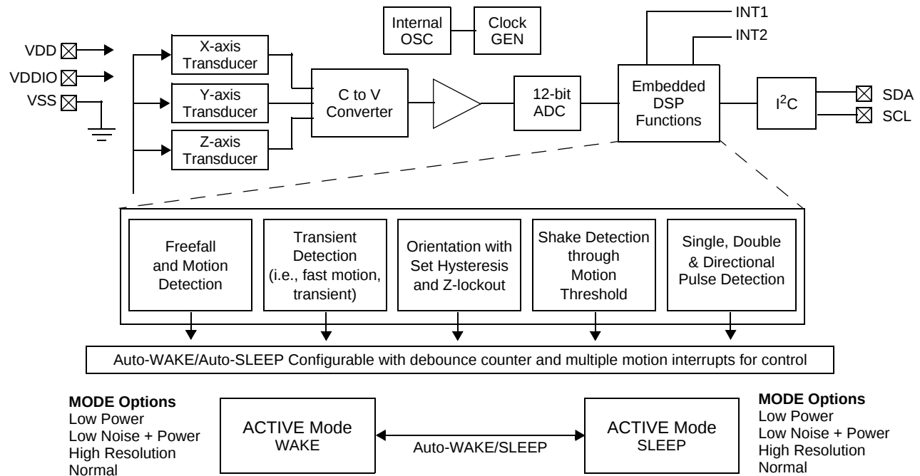
Figure 1. Block Diagram
