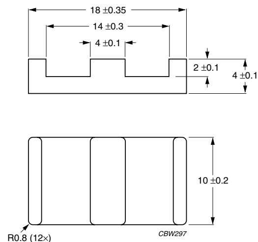
Fig.1 E18/4/10 core half.
