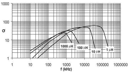
Typical Q vs Frequency (f)
