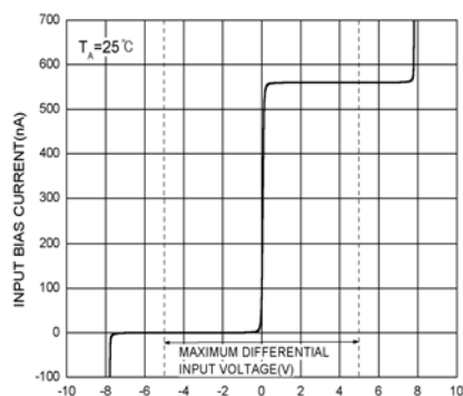
Figure 6. Input Characteristics
