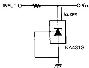
Figure 3. Test Circuit for I_{KA}(\text{OFF})
