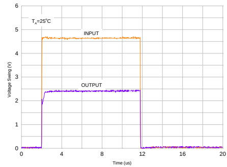
Figure 9. Pulse Response
