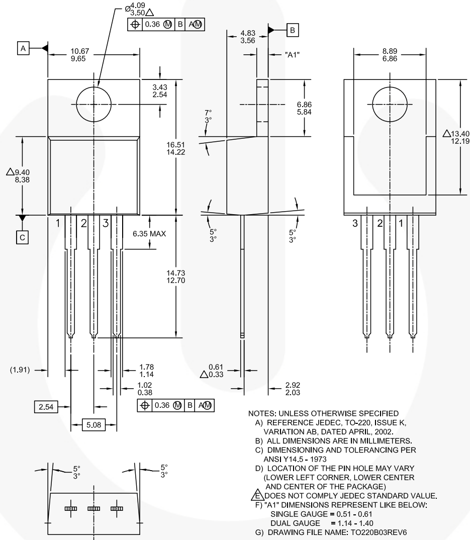
Figure 9. TO220, MOLDED, 3-LEAD, JEDEC VARIATION (ACTIVE)
