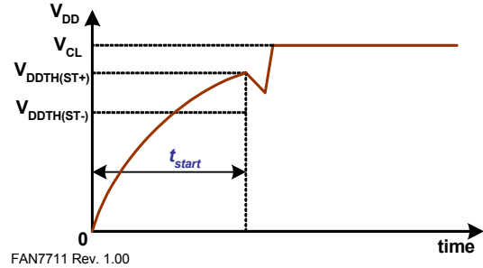
Figure 27. V_{DD} Build-up
