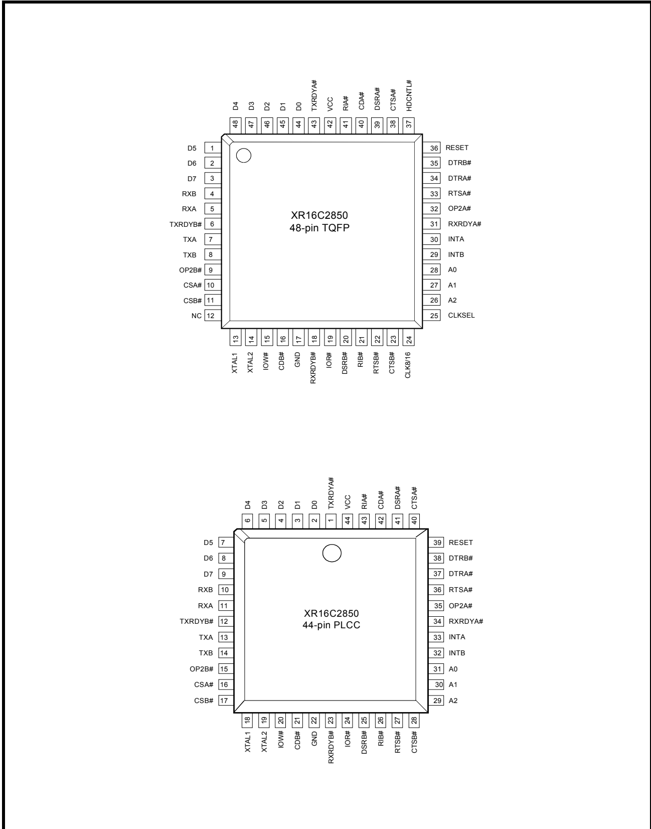
FIGURE 2. PIN OUT ASSIGNMENT
