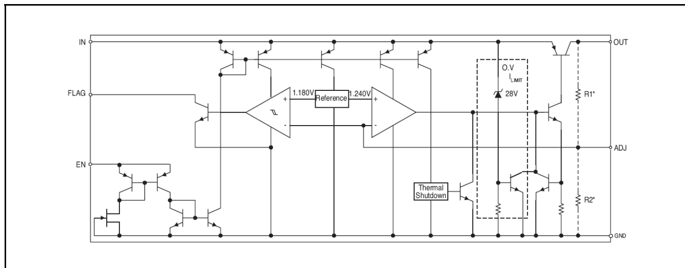
Fig. 2: XRP29300/01/02 Block Diagram
