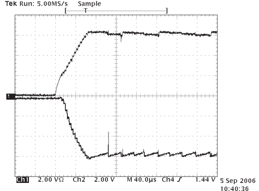
SP3224E/SP3226E Charge Pump Power On Time, V_{CC}=3.3V
