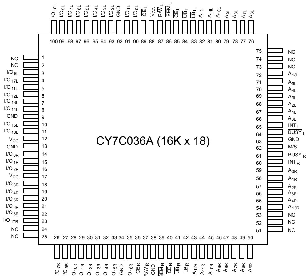
100-Pin TQFP Top View
