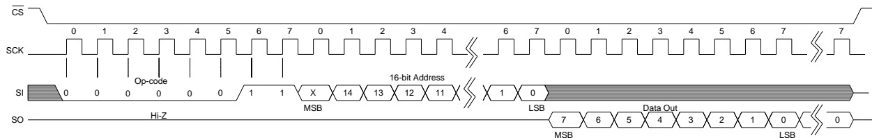
Figure 23. Memory Read
