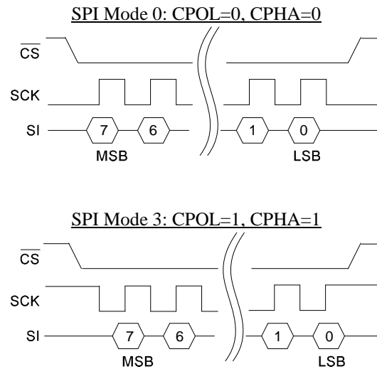
Figure 15. SPI Modes 0 & 3
