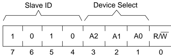
Figure 4. Slave Address
