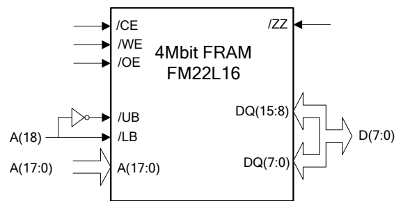
Figure 4. FM22L16 Wired as 512Kx8
