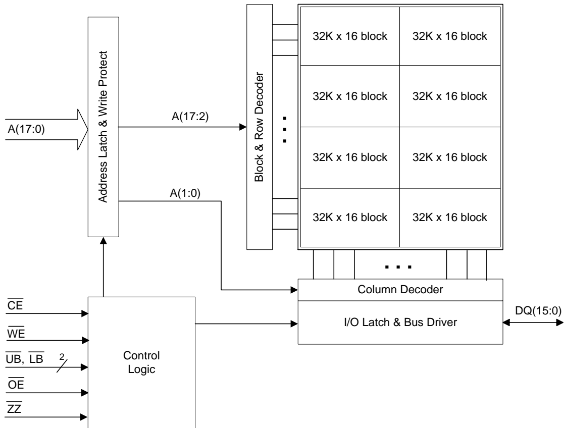
Figure 1. Block Diagram
