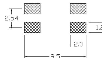
PCB PATTERN
