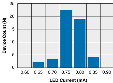
PLA132 Typical I F for Switch Operation Ambient Temperature = 25°C Load Current = 600mA
