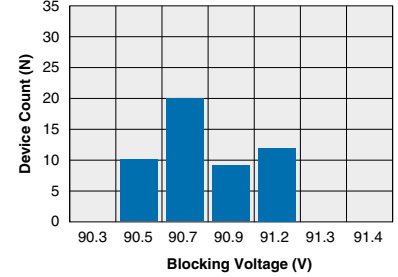
PLA132 Typical Blocking Voltage Distribution (N=50 Ambient Temperature = 25°C)
