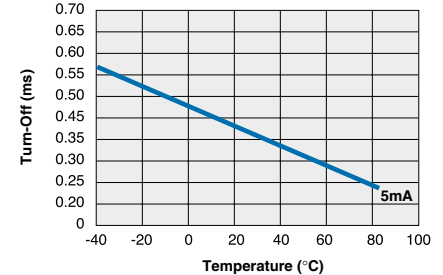
PLA132 Typical Turn-Off vs. Temperature Load Current = 600mA
