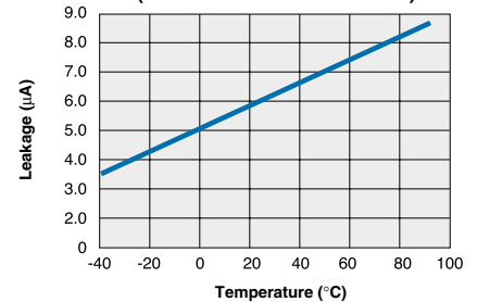
PLA132 Leakage vs. Temperature (Measured Across Pins 6 & 4)
