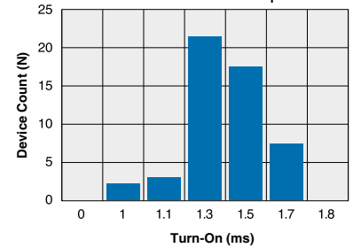
PLA132 Typical Turn-On Time (N=50 Ambient Temperature = 25°C) Load Current = 600mA I F = 5mA
