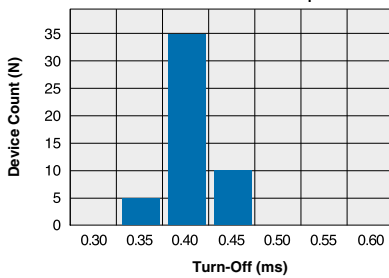
PLA132 Typical Turn-Off Time (N=50 Ambient Temperature = 25°C) Load Current = 600mA I F = 5mA
