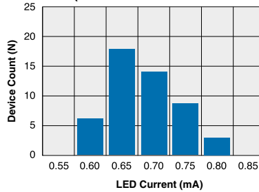
PLA132 Typical I F for Switch Dropout (N=50 Ambient Temperature = 25°C) (Load Current = 120mADC)
