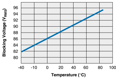
PLA132 Typical Blocking Voltage vs. Temperature
