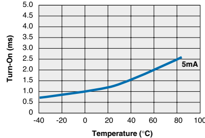
PLA132 Typical Turn-On vs. Temperature Load Current = 600mA
