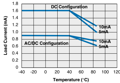
PLA132 Maximum Load Current vs. Temperature
