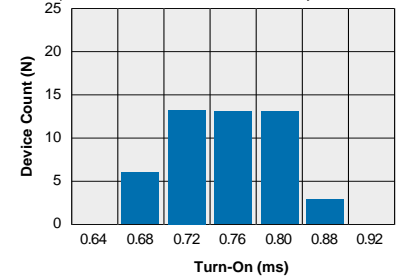
PAA193 Typical Turn-On Time (N=50 Ambient Temperature = 25°C) (Load Current = 120mADC; I_F = 5\text{mADC} )
