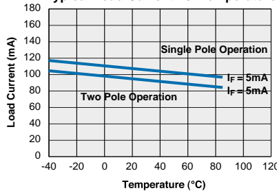
PAA193 Typical Load Current vs. Temperature
