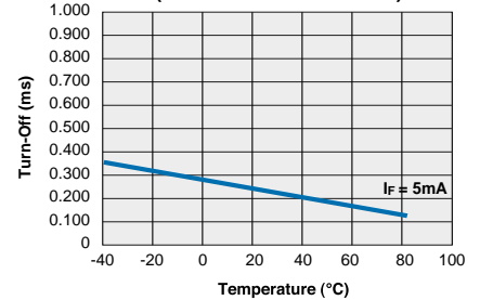
PAA193 Typical Turn-Off vs. Temperature (Load Current = 50mADC)
