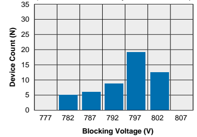
PAA193 Typical Blocking Voltage Distribution (N=50 Ambient Temperature = 25°C)
