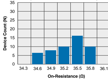
PAA193 Typical On-Resistance Distribution (N=50 Ambient Temperature = 25°C) (Load Current = 120mADC)
