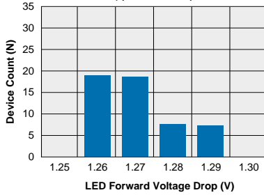
PAA193 Typical LED Forward Voltage Drop (N=50 Ambient Temperature = 25°C) ( I_F = 5\text{mADC} )
