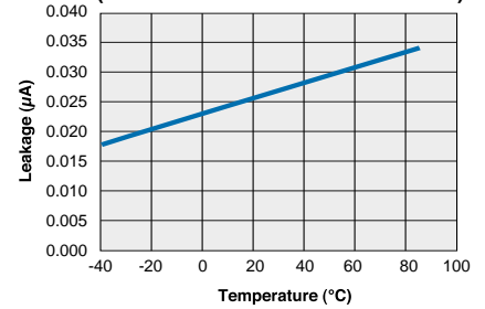
PAA193 Typical Leakage vs. Temperature (Measured across Pins 5 & 6 or 7 & 8)
