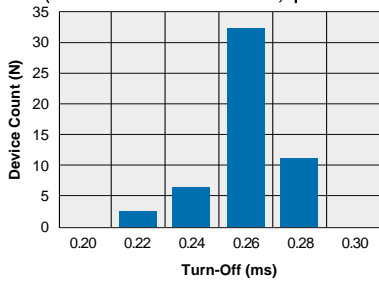
PAA193 Typical Turn-Off Time (N=50 Ambient Temperature = 25°C) (Load Current = 120mADC; I_F = 5\text{mADC} )
