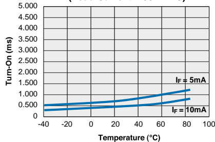
PAA193 Typical Turn-On vs. Temperature (Load Current = 50mADC)
