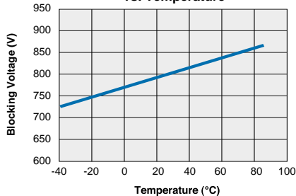
PAA193 Typical Blocking Voltage vs. Temperature
