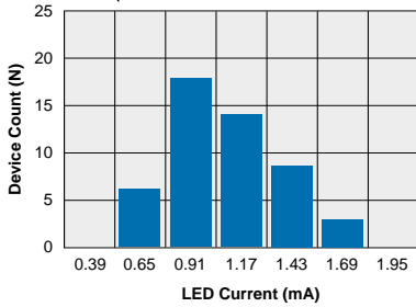
PAA193 Typical I_F for Switch Dropout (N=50 Ambient Temperature = 25°C) (Load Current = 120mADC)
