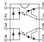
LDA210 Pinout
