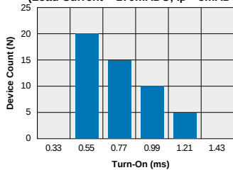
LBA127L - Form A Typical Turn-On Time (N=50 Ambient Temperature = 25°C) (Load Current = 170mADC; I_F = 5mADC)
