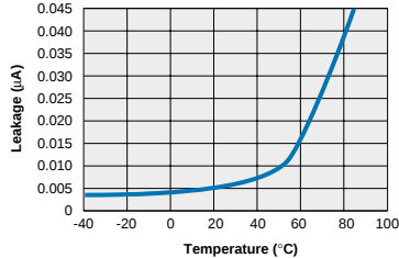
LBA127L Typical Leakage vs. Temperature (Measured across Pins 5 & 6 or 7 & 8)
