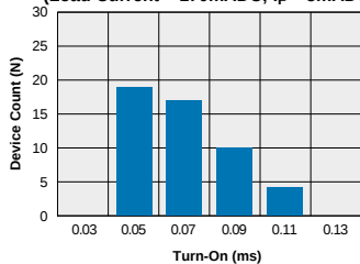
LBA127L - Form B Typical Turn-On Time (N=50 Ambient Temperature = 25°C) (Load Current = 170mADC; I_F = 5mADC)
