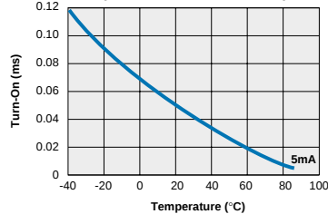
LBA127L - Form B Typical Turn-On vs. Temperature (Load Current = 170mADC)
