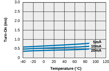
LBA127L - Form A Typical Turn-On vs. Temperature (Load Current = 170mADC)
