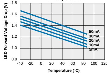
LBA127L Typical LED Forward Voltage Drop vs. Temperature
