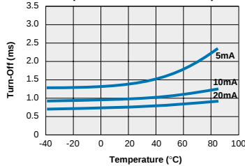
LBA127L - Form B Typical Turn-Off vs. Temperature (Load Current = 170mADC)
