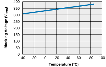
LBA127L - Form B Typical Blocking Voltage vs. Temperature
