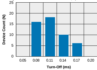
LBA127L - Form A Typical Turn-Off Time (N=50 Ambient Temperature = 25°C) (Load Current = 170mADC; I_F = 5mADC)
