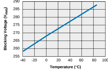
LBA127L - Form A Typical Blocking Voltage vs. Temperature
