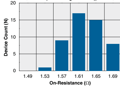
Typical On-Resistance (N=50, I_F=0\text{mA} , I_L=5\text{mA} , T_A=25^\circ\text{C} )
