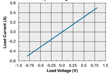
Typical Load Voltage vs. Load Current ( I_F=0mA, T_A=25°C )
