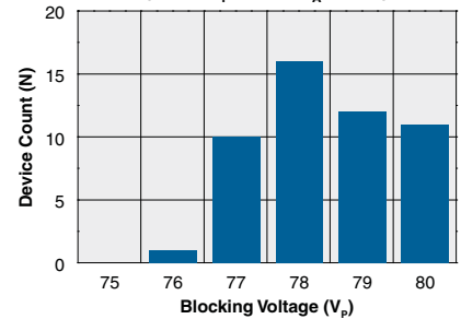
Typical Blocking Voltage (N=50, I_F=2\text{mA} , T_A=25^\circ\text{C} )
