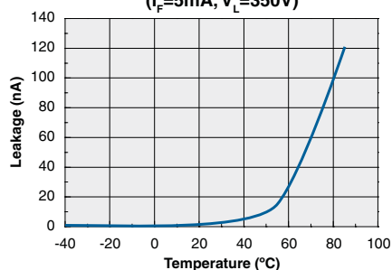
Leakage Current vs. Temperature Measured Across Pins 7 & 8 ( I_F=5\text{mA} , V_L=350\text{V} )
