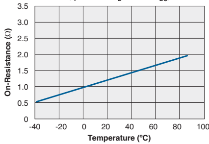
Typical On-Resistance vs. Temperature ( I_F=10\text{mA} , I_L=100\text{mA}_{\text{DC}} )
