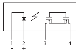
CPC1916Y Pinout
