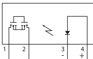
CPC1908J Pinout
