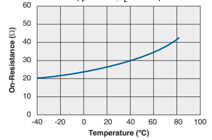
Typical On-Resistance vs. Temperature ( I_F=10mA, I_L=80mA )
