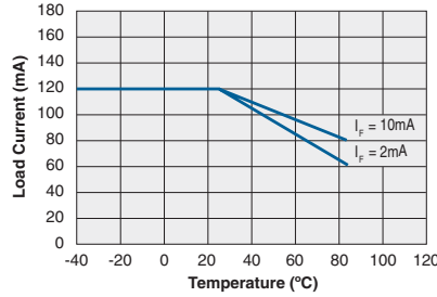
Typical Load Current vs. Temperature
