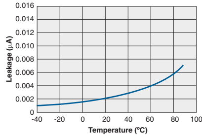
Typical Leakage vs. Temperature Measured Across Pins 3 & 4
