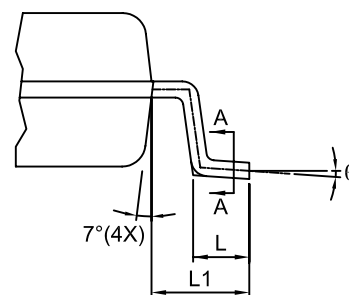
DETAIL "A" (2:1)
