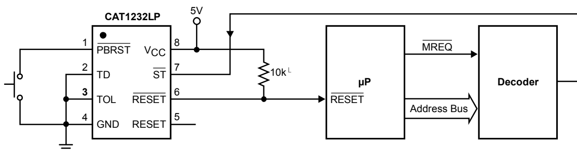
Figure 5. CAT1232LP Application Circuit: Watchdog Timer
