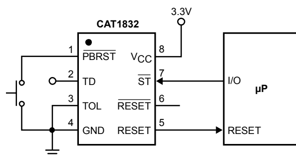
Figure 4. CAT1832 Application Circuit: Pushbutton Reset
