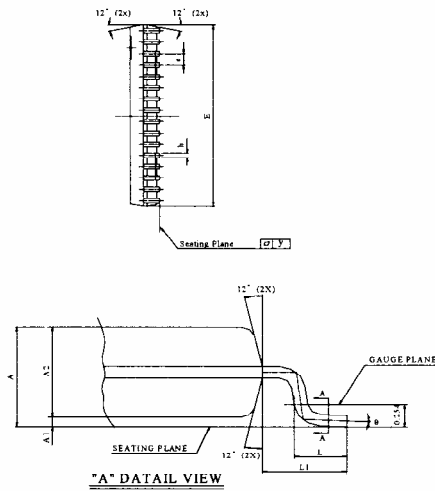
"A" DETAIL VIEW
