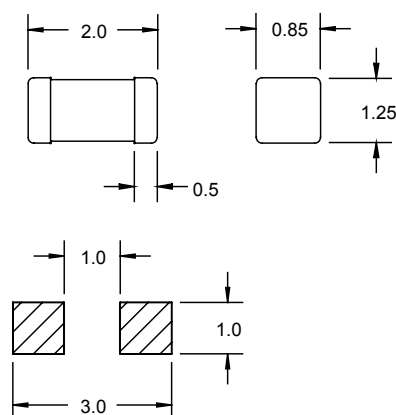
Pad Layout
