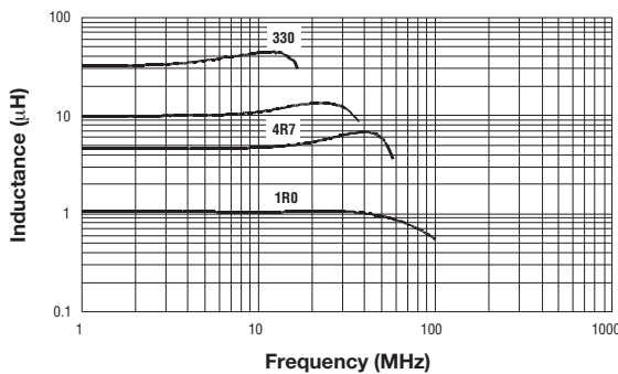
Inductance Characteristics
