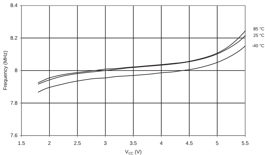
Figure 20-50. Frequency of Calibrated 8.0 MHz Oscillator vs. Temperature
