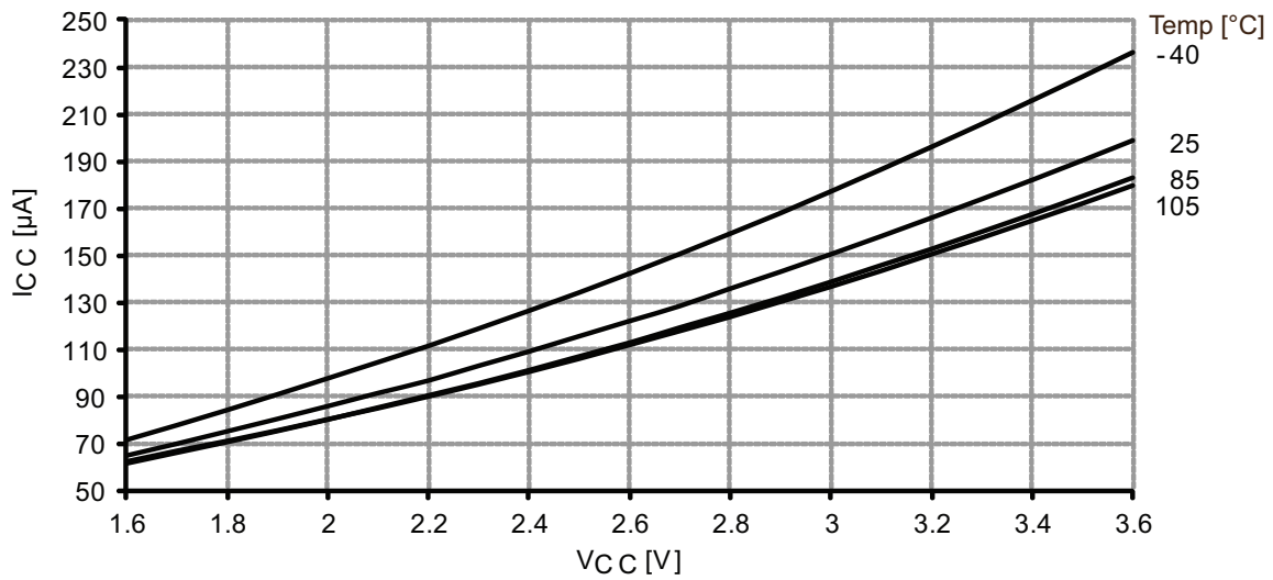
Figure 37-3. Active mode supply current vs. V_{CC} . f_{SYS} = 32.768kHz internal oscillator.
