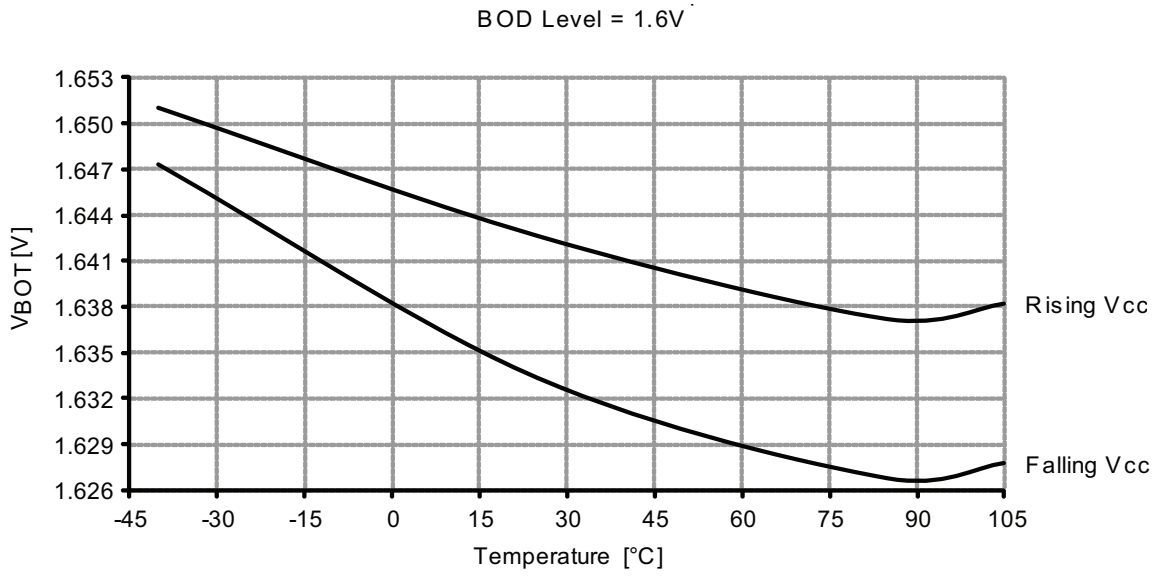
Figure 37-59. BOD thresholds vs. temperature.
