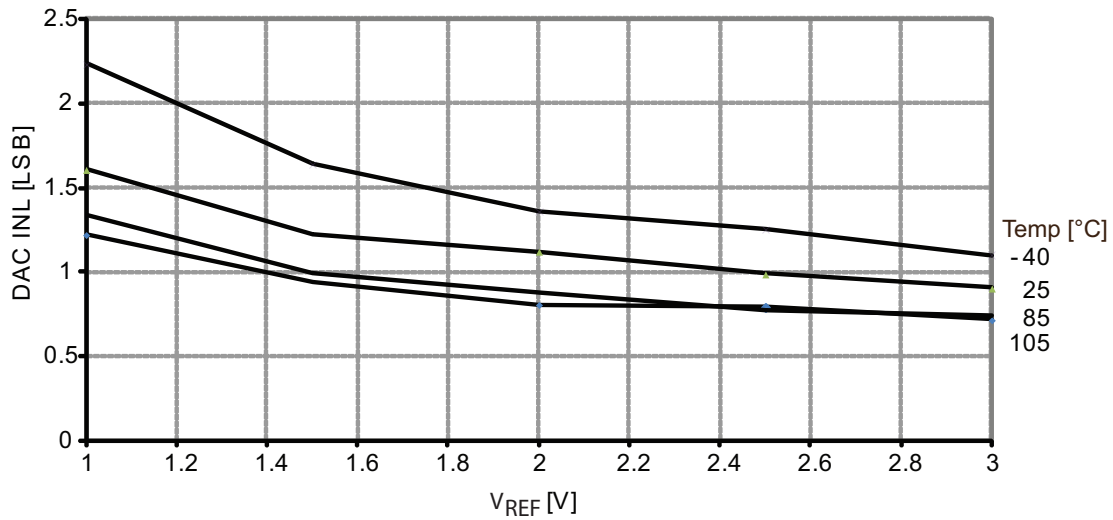
Figure 37-48. DAC INL error vs. V_{REF} . V_{CC} = 3.6\text{V} .
