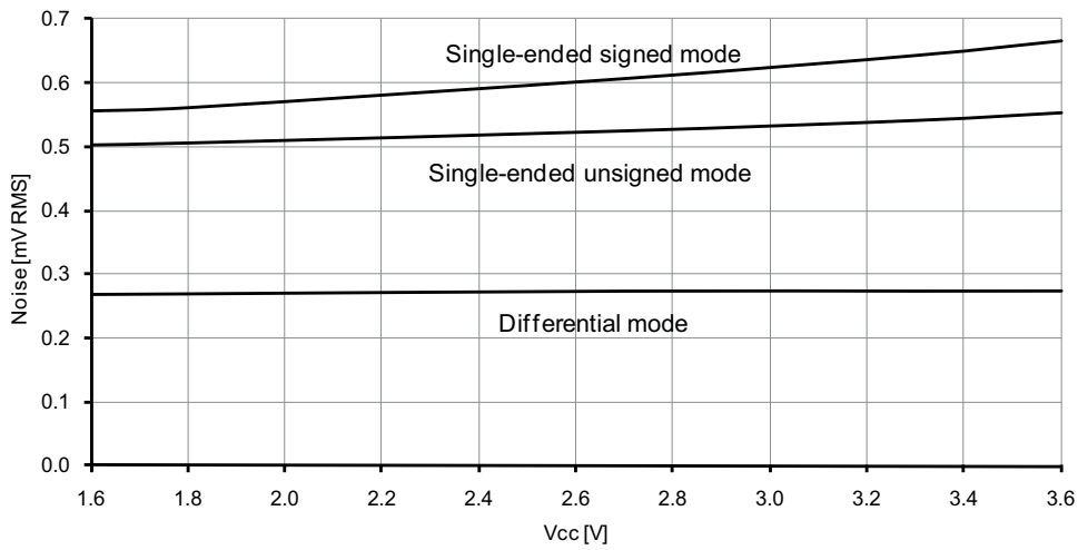
Figure 37-47. Noise vs. V_{CC} . T = 25^{\circ}\text{C} , V_{REF} = \text{external } 1.0\text{V} , ADC sampling speed = 500ksps.
