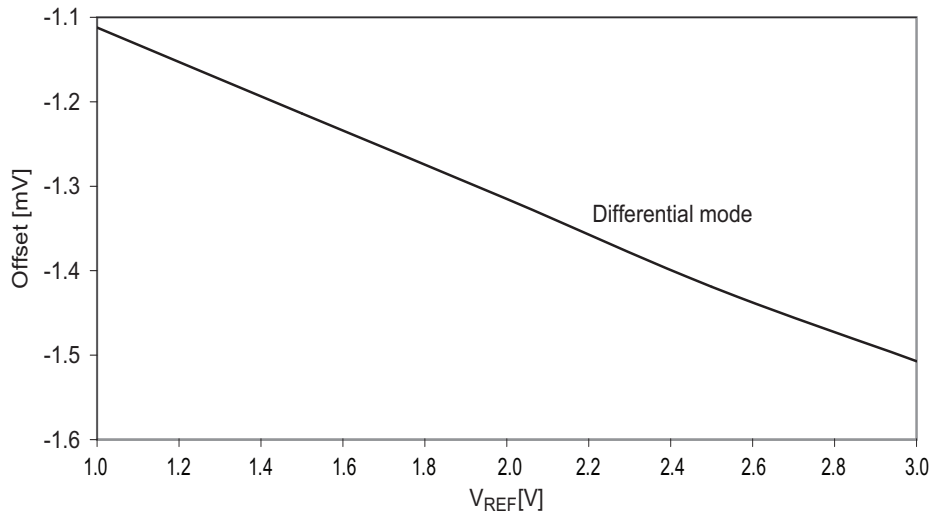
Figure 37-209. Offset error vs. V_{REF} .
