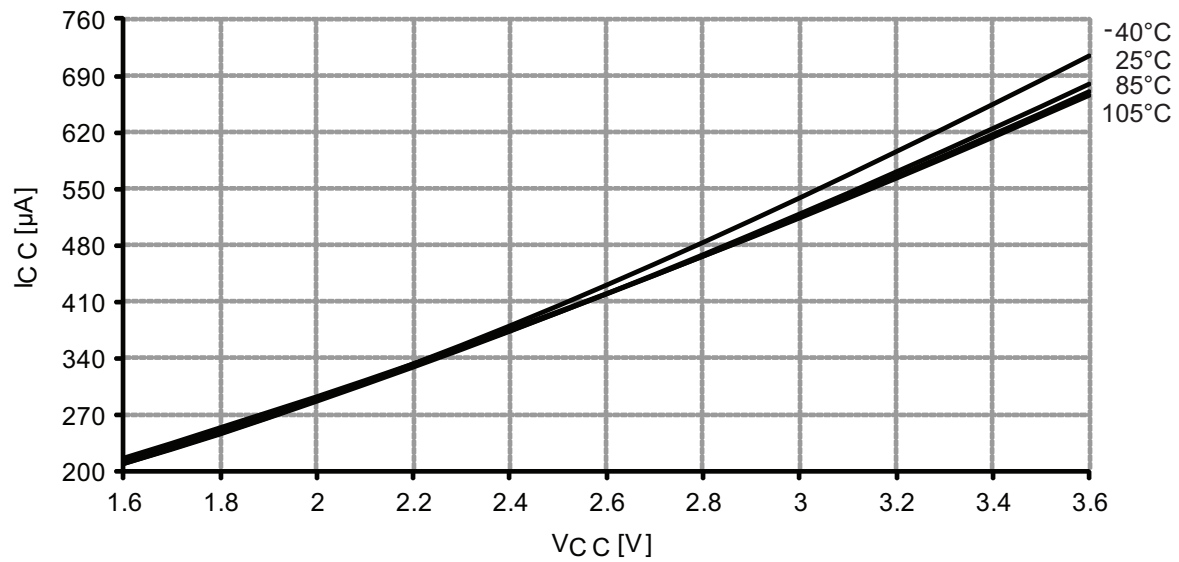
Figure 37-4. Active mode supply current vs. V_{CC} . f_{SYS} = 1MHz external clock.
