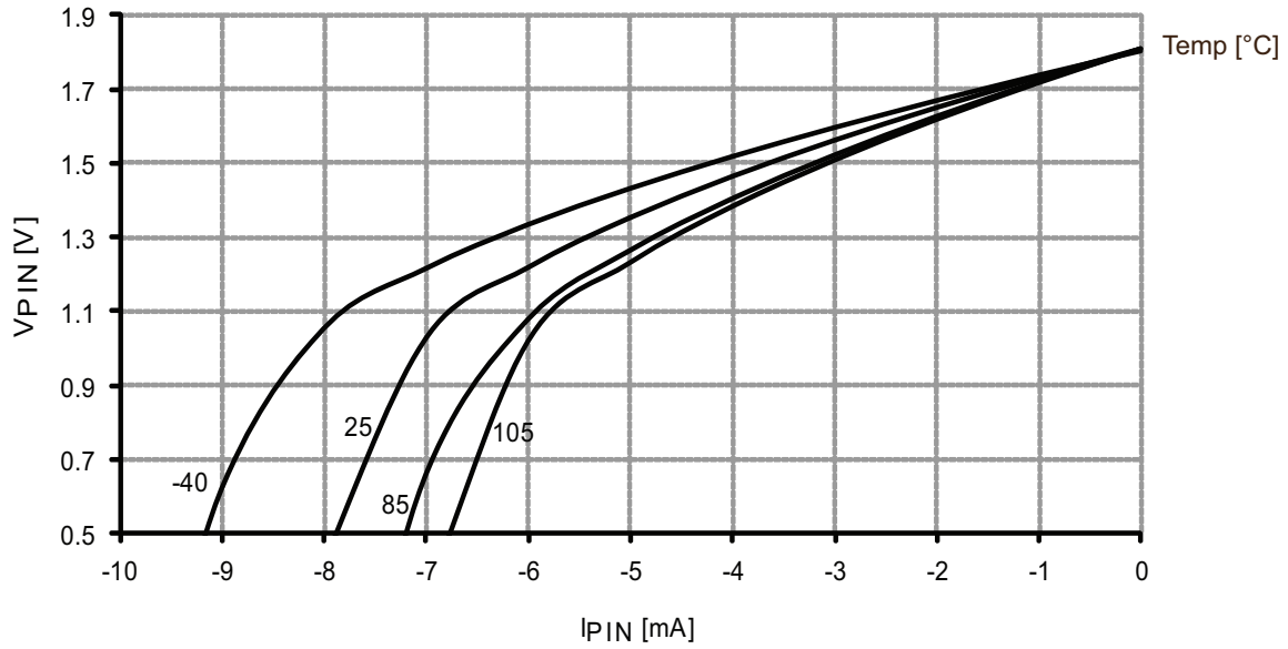
Figure 37-23. I/O pin output voltage vs. source current. V_{CC} = 1.8V.
