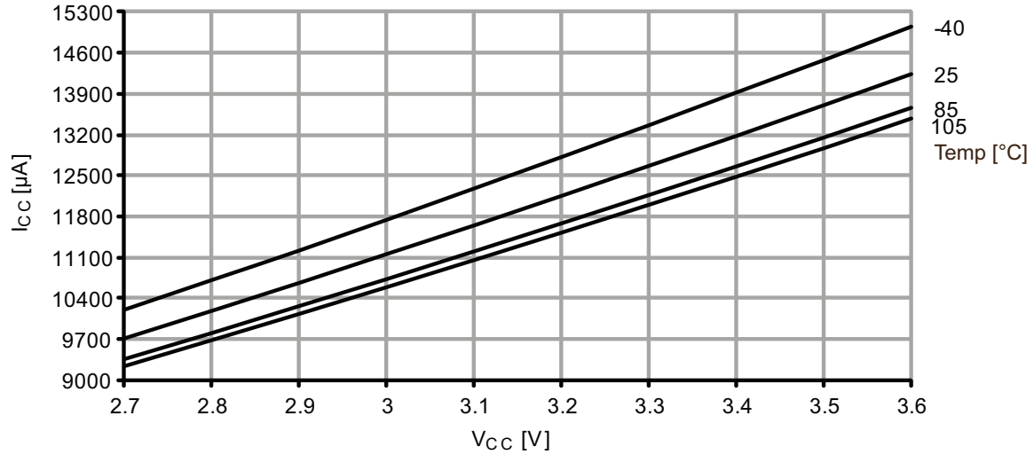
Figure 37-90. Active mode supply current vs. V_{CC} .
