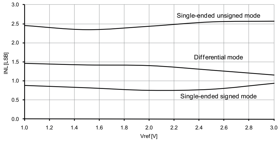
Figure 37-118. INL error vs. external V_{REF} . T = 25^\circ\text{C} , V_{CC} = 3.6\text{V} , external reference.
