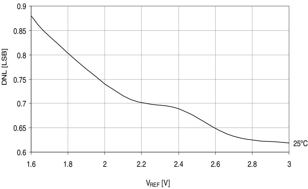
Figure 37-303.DNL error vs. V_{REF} . T = 25^{\circ}C , V_{CC} = 3.6V .
