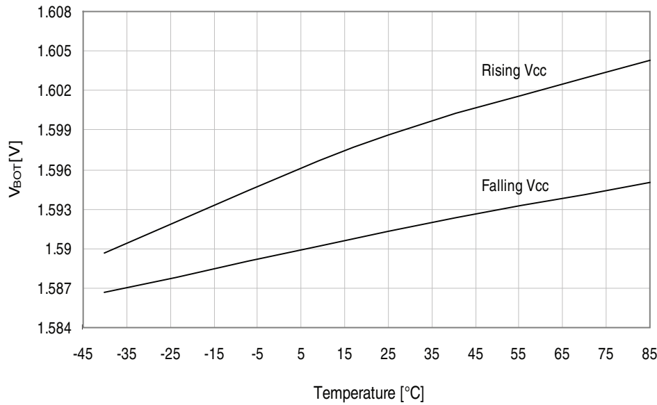
Figure 37-230.BOD thresholds vs. temperature.
