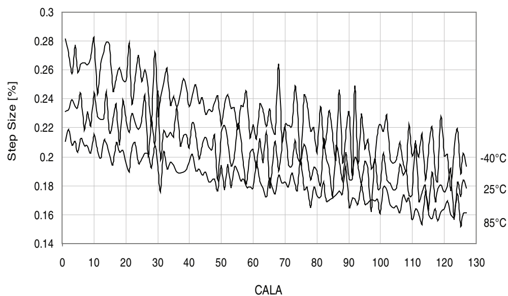
Figure 37-328. 2MHz internal oscillator CALA calibration step size.
