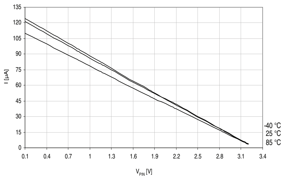
Figure 37-108. I/O pin pull-up resistor current vs. input voltage.
