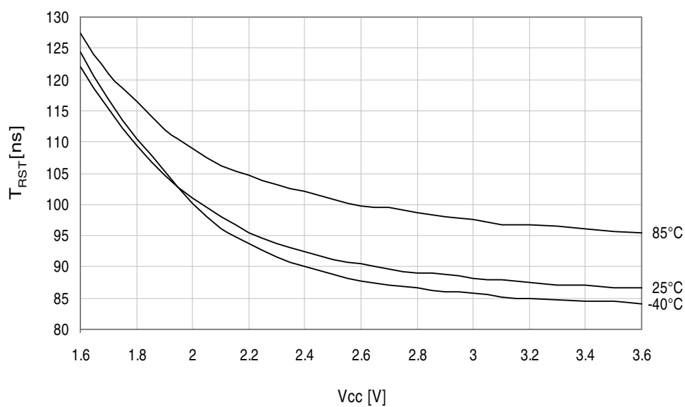
Figure 37-232. Minimum Reset pin pulse width vs. V_{CC} .
