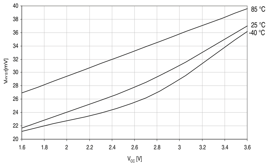
Figure 37-139. Analog comparator hysteresis vs. V_{CC} . High-speed mode, large hysteresis.
