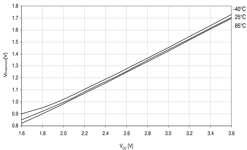
Figure 37-118. I/O pin input threshold voltage vs. V_{CC} .
