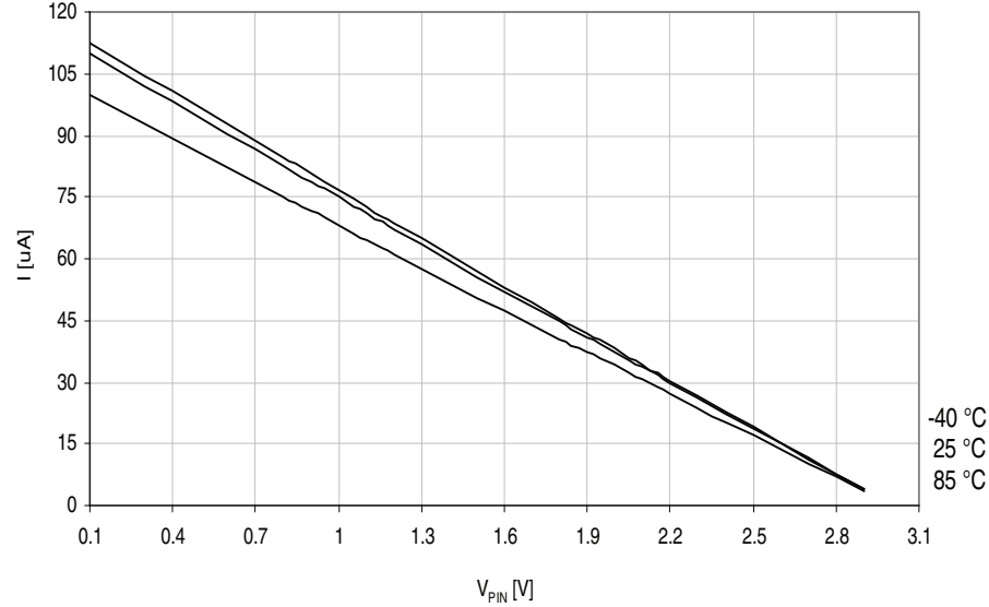
Figure 37-107. I/O pin pull-up resistor current vs. input voltage. V_{CC} = 3.0V .
