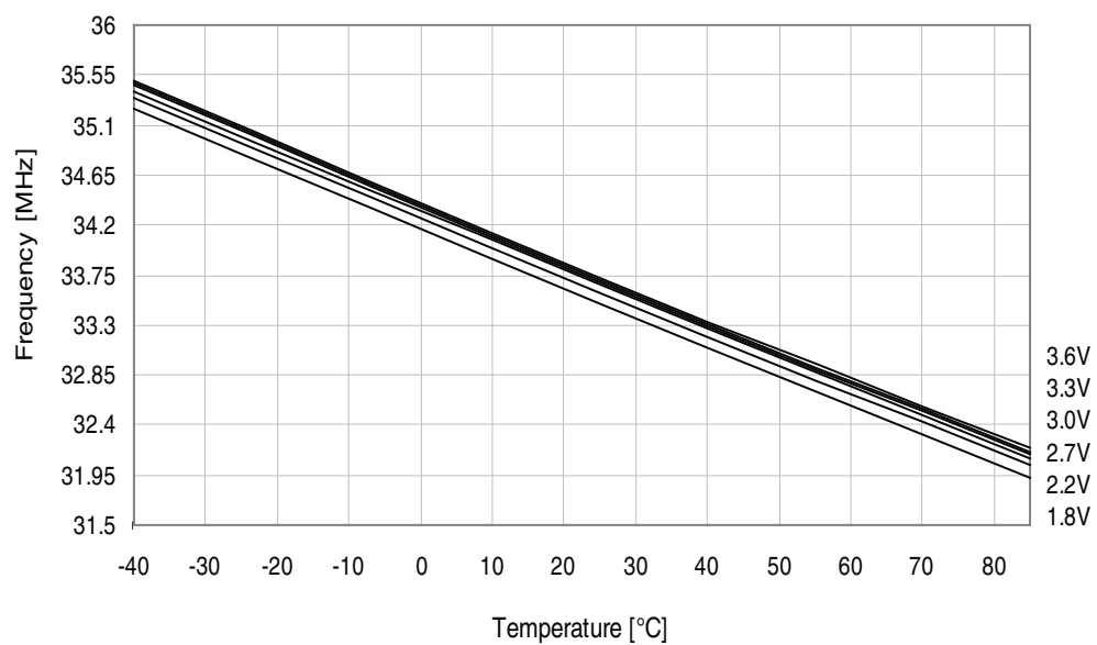
Figure 37-329. 32MHz internal oscillator frequency vs. temperature.
