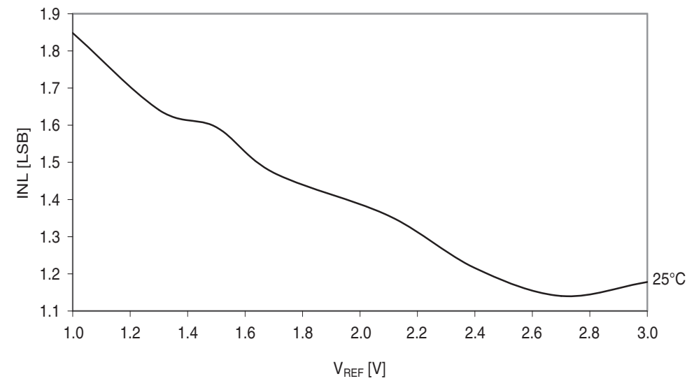
Figure 37-219.DAC INL error vs. V_{REF} . V_{CC} = 3.6V .
