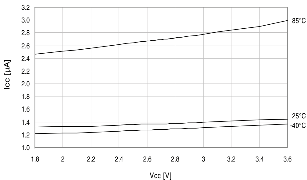
Figure 37-270. Power-down mode supply current vs. V_{CC} . Watchdog and sampled BOD enabled.
