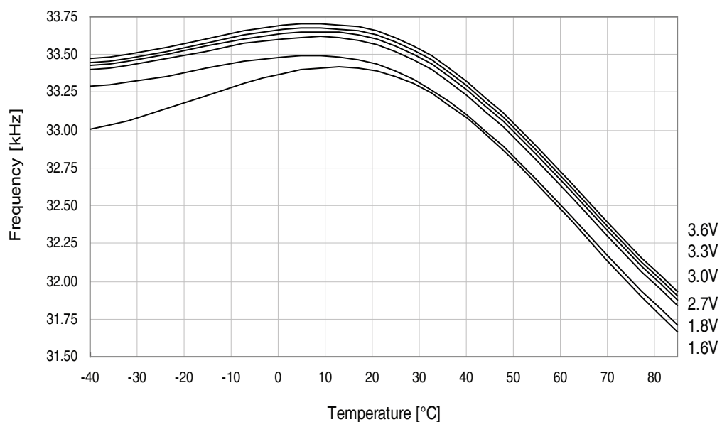
Figure 37-240. Ultra Low-Power internal oscillator frequency vs. temperature.
