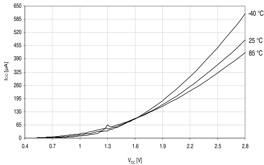
Figure 37-322. Power-on reset current consumption vs. V_{CC} . BOD level = 3.0V, enabled in sampled mode.
