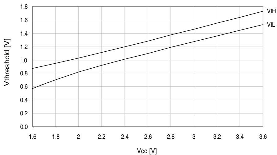
Figure 37-202. I/O pin input threshold voltage vs. V_{CC} . T = 25^{\circ}\text{C} .
