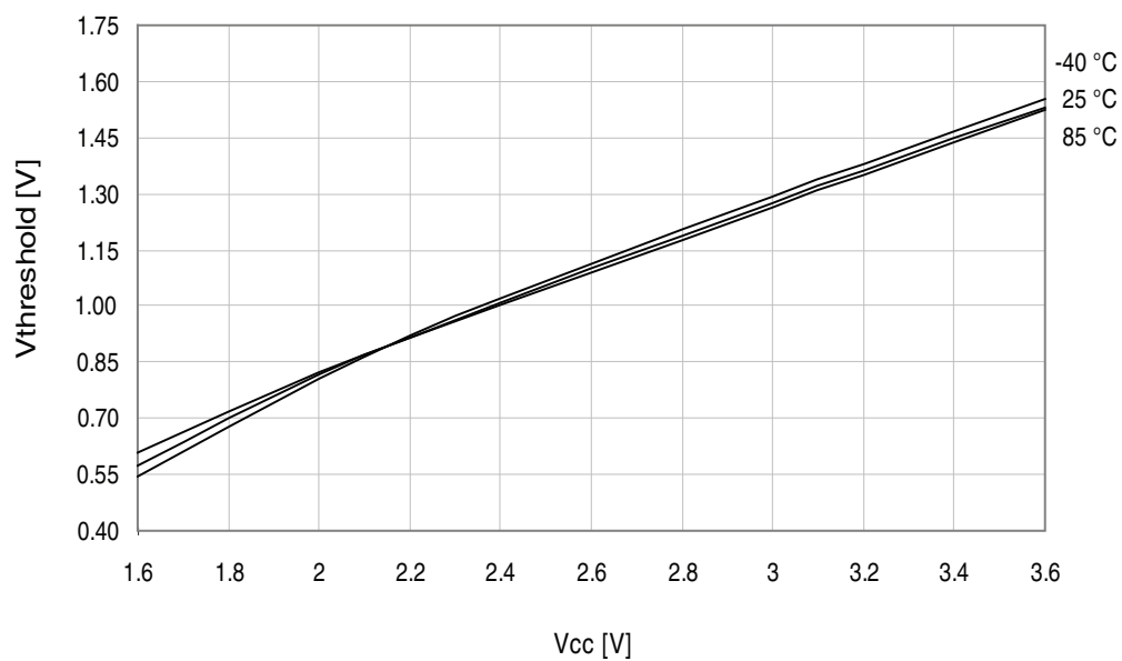
Figure 37-287. I/O pin input threshold voltage vs. V_{CC} .
