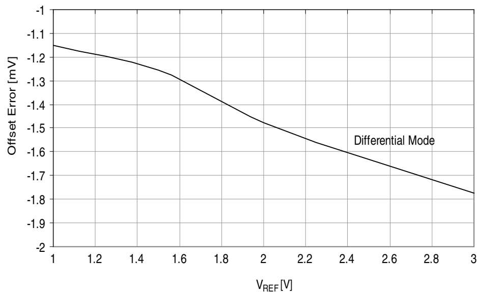
Figure 37-214. Offset error vs. V_{REF} .
