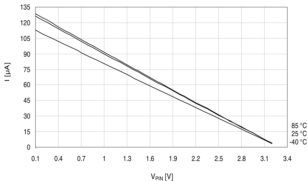
Figure 37-193. I/O pin pull-up resistor current vs. input voltage.
