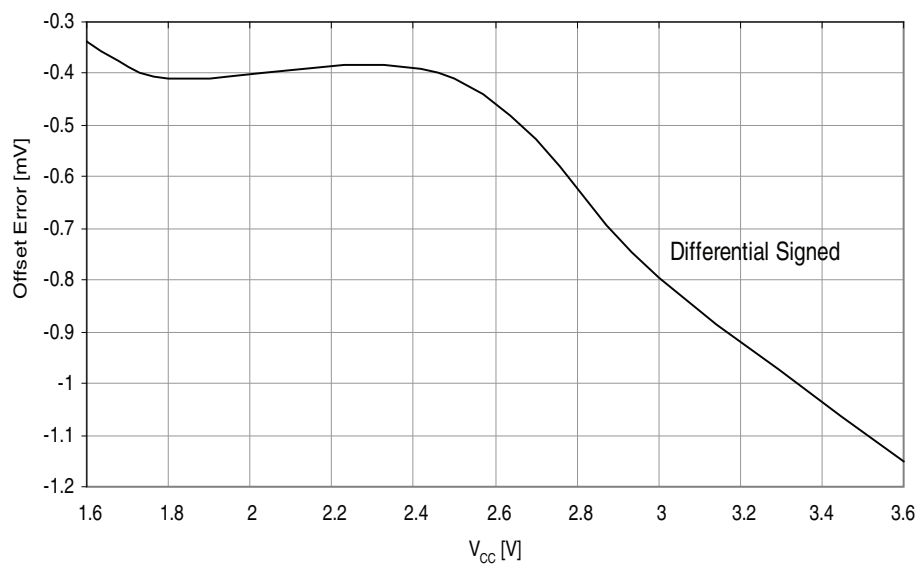
Figure 37-299. Offset error vs. V_{CC} .
