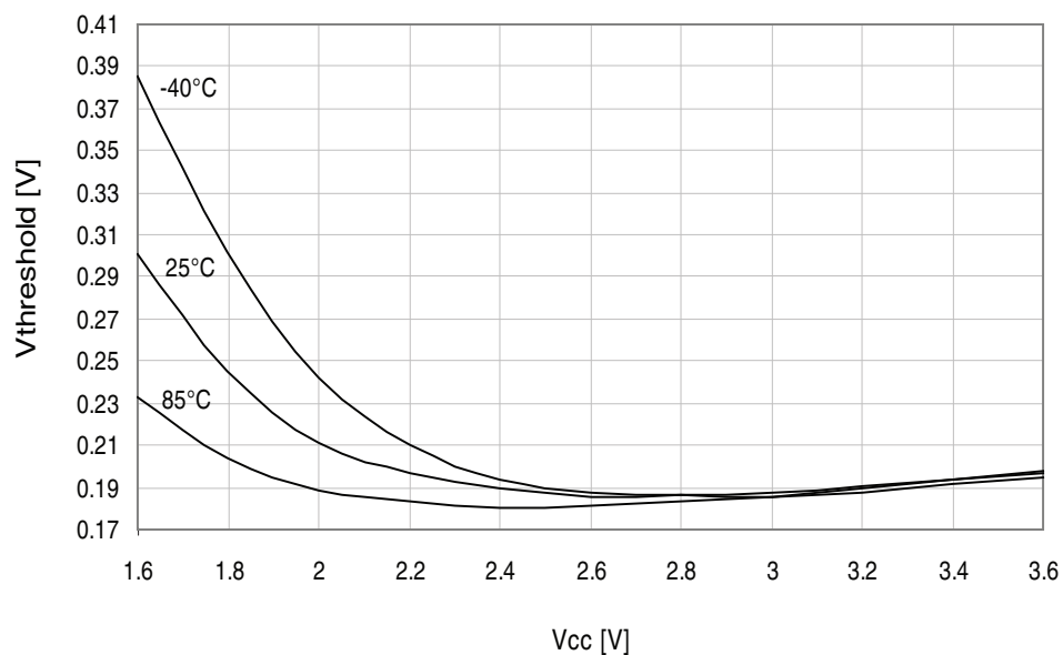
Figure 37-288. I/O pin input hysteresis vs. V_{CC} .
