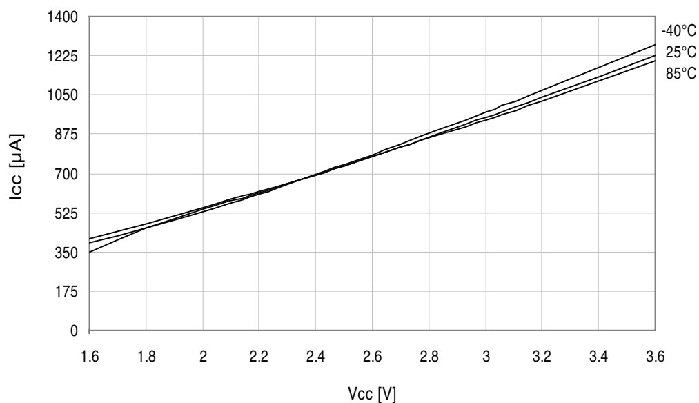
Figure 37-176. Active mode supply current vs. V_{CC} .
