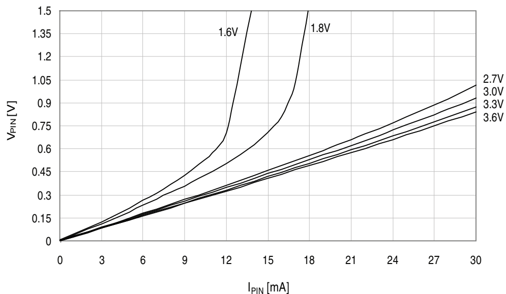
Figure 37-201. I/O pin output voltage vs. sink current.
