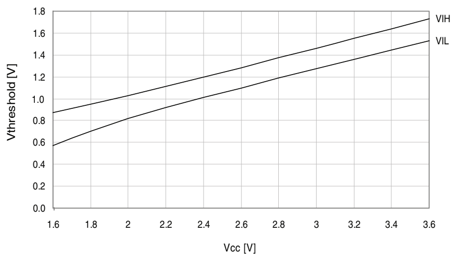
Figure 37-117. I/O pin input threshold voltage vs. V_{CC} .
