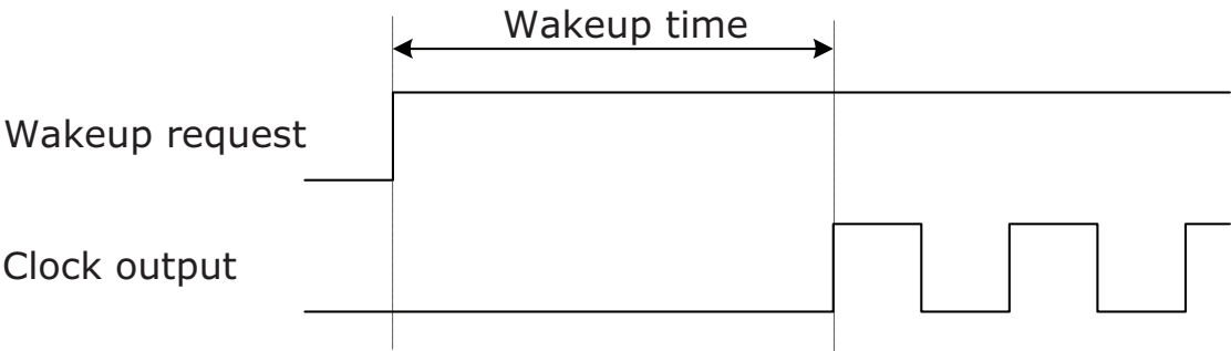
Figure 36-23.Wake-up time definition.
