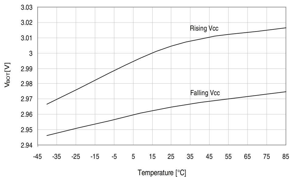
Figure 37-314. BOD thresholds vs. temperature.
