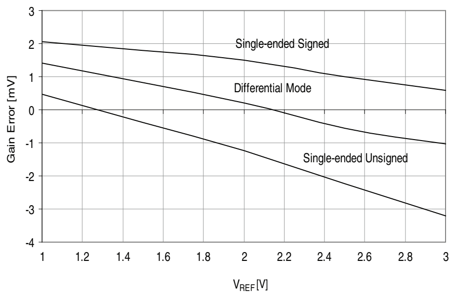
Figure 37-295.Gain error vs. V_{REF} .
