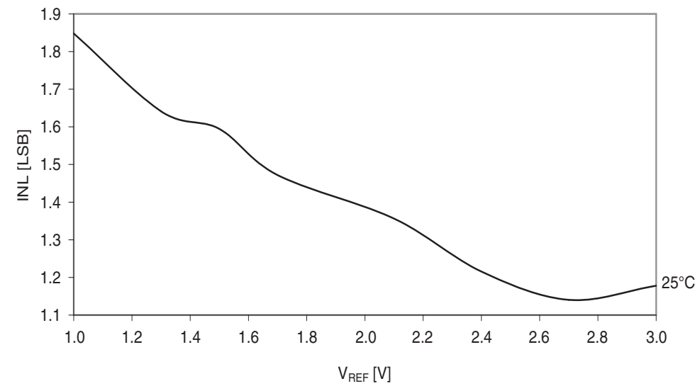
Figure 37-302.DAC INL error vs. V_{REF} . V_{CC} = 3.6V .
