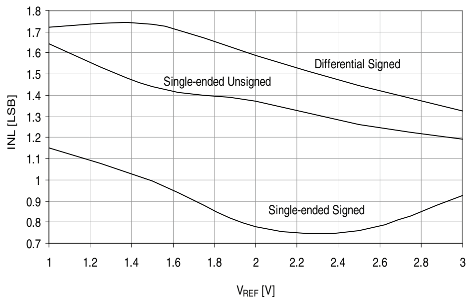
Figure 37-289. INL error vs. external V_{REF} .
