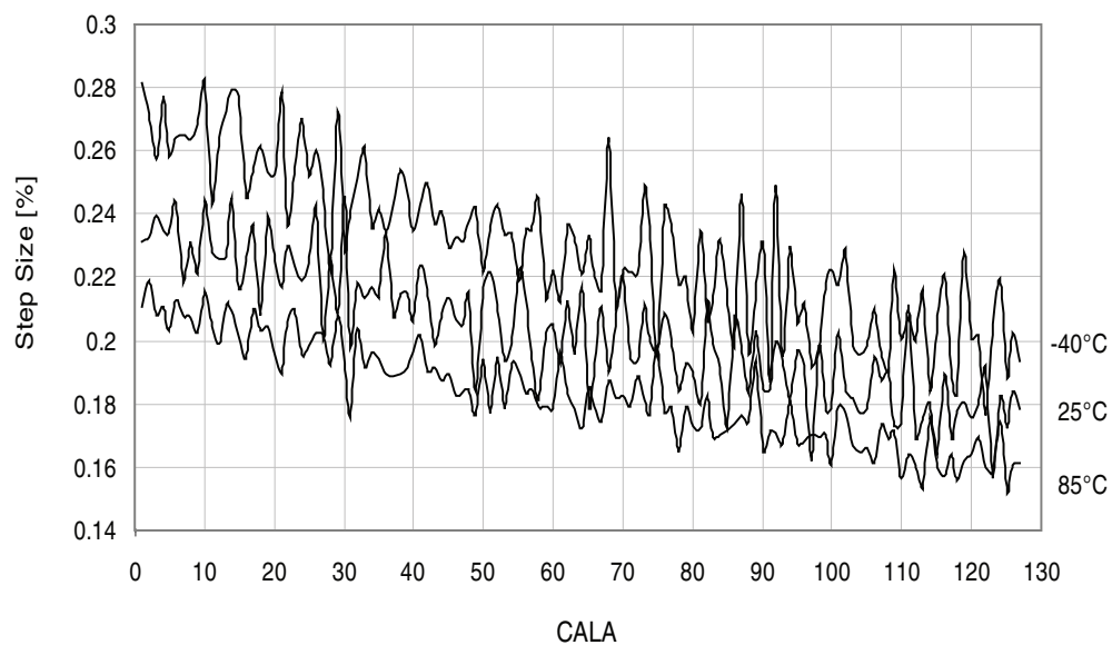
Figure 37-245. 2MHz internal oscillator CALA calibration step size.
