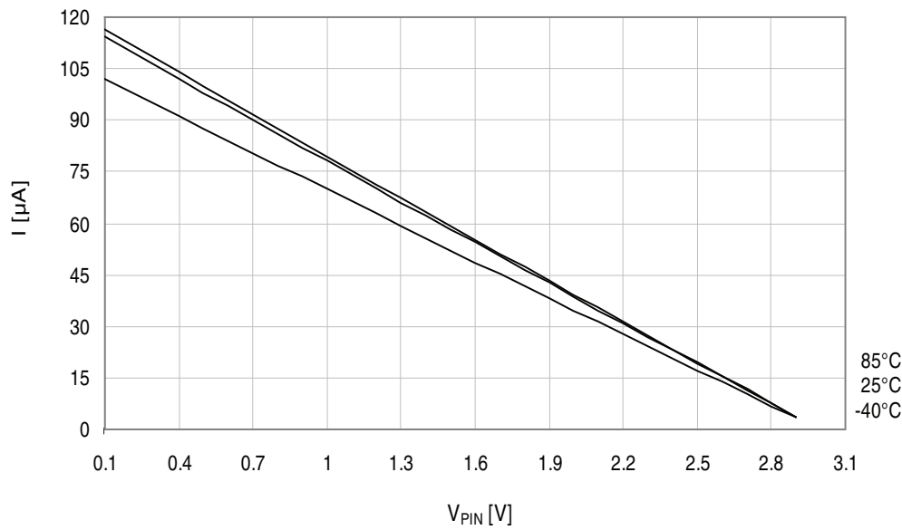
Figure 37-192. I/O pin pull-up resistor current vs. input voltage. V_{CC} = 3.0V .
