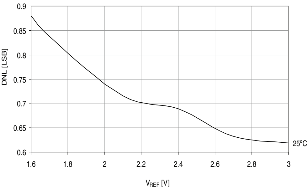
Figure 37-220.DNL error vs. V_{REF} . T = 25^{\circ}C , V_{CC} = 3.6V .
