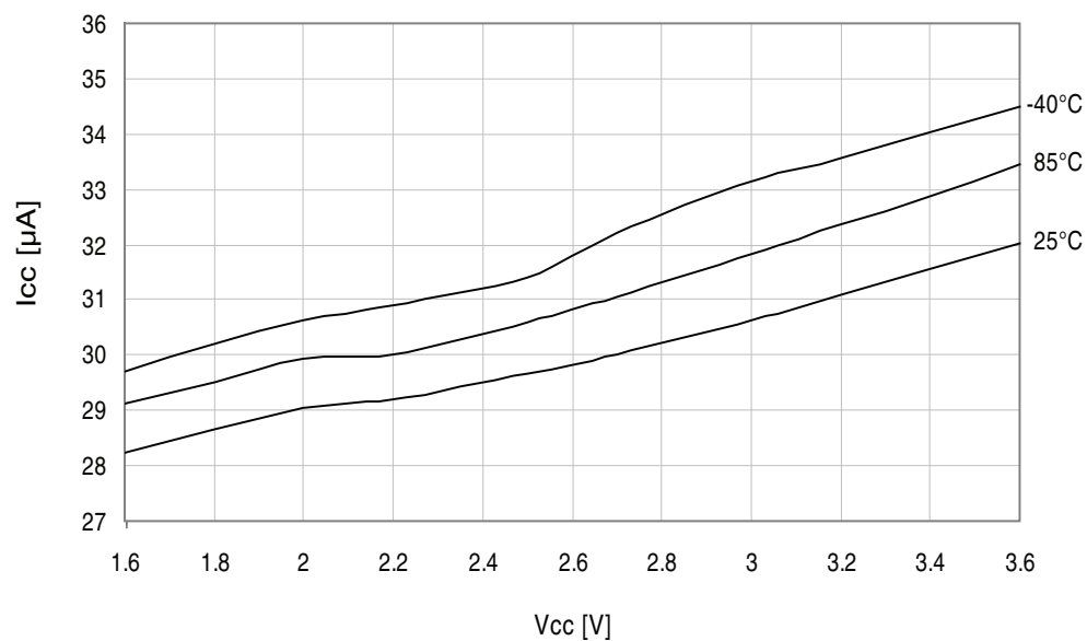
Figure 37-180. Idle mode supply current vs. V_{CC} .
