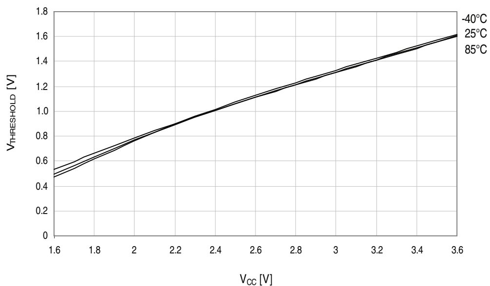
Figure 37-320. Reset pin input threshold voltage vs. V_{CC} .
