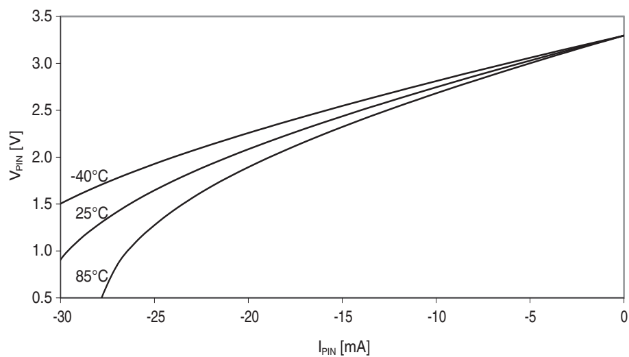
Figure 37-111. I/O pin output voltage vs. source current.
