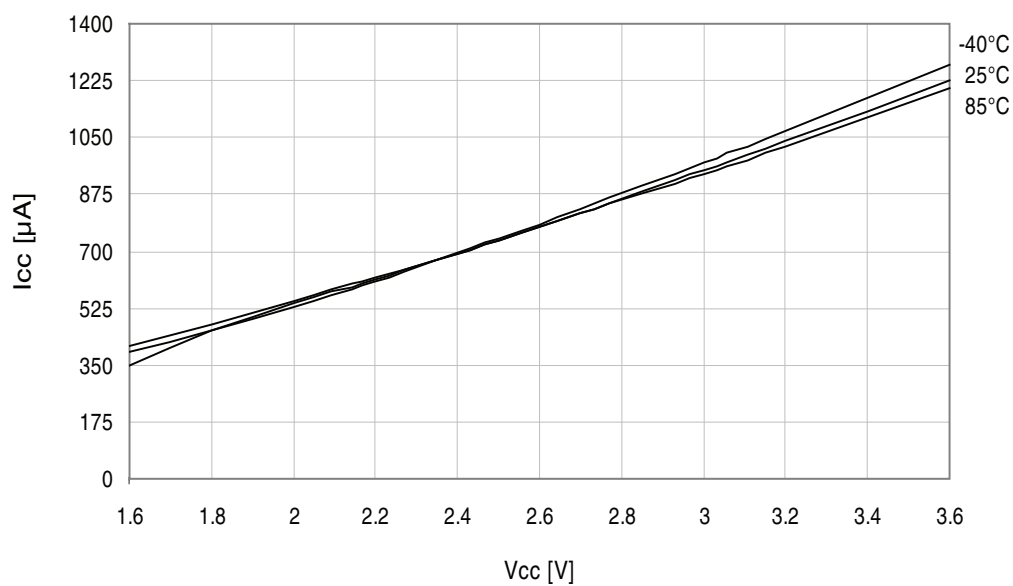
Figure 37-259. Active mode supply current vs. V_{CC} .
