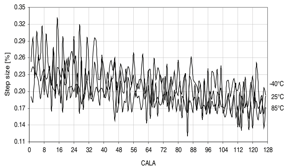
Figure 37-82. 48MHz internal oscillator CALA calibration step size. V_{CC} = 3.0V .
