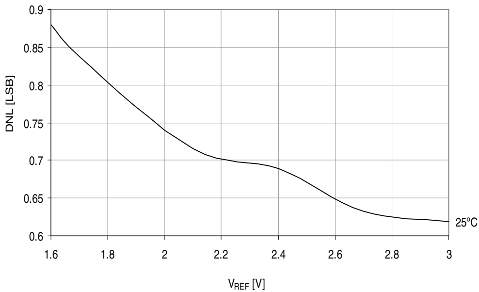
Figure 37-50.DNL error vs. V_{REF} . T = 25^{\circ}C , V_{CC} = 3.6V .
