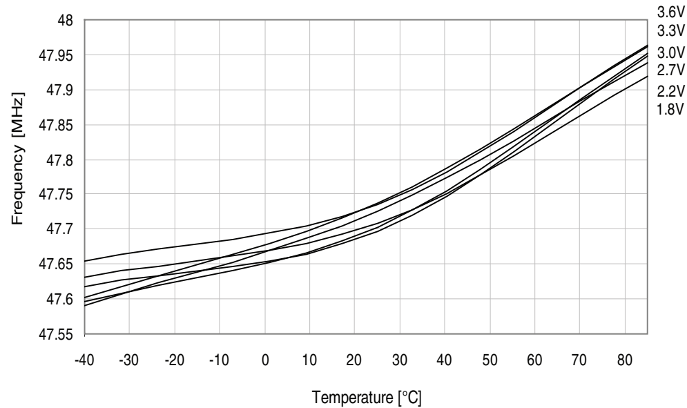
Figure 37-333.48MHz internal oscillator frequency vs. temperature. DPLL enabled, from the 32.768kHz internal oscillator.
