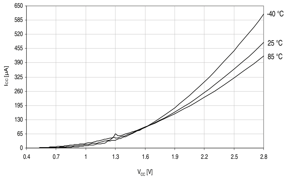
Figure 37-154. Power-on reset current consumption vs. V_{CC} .
