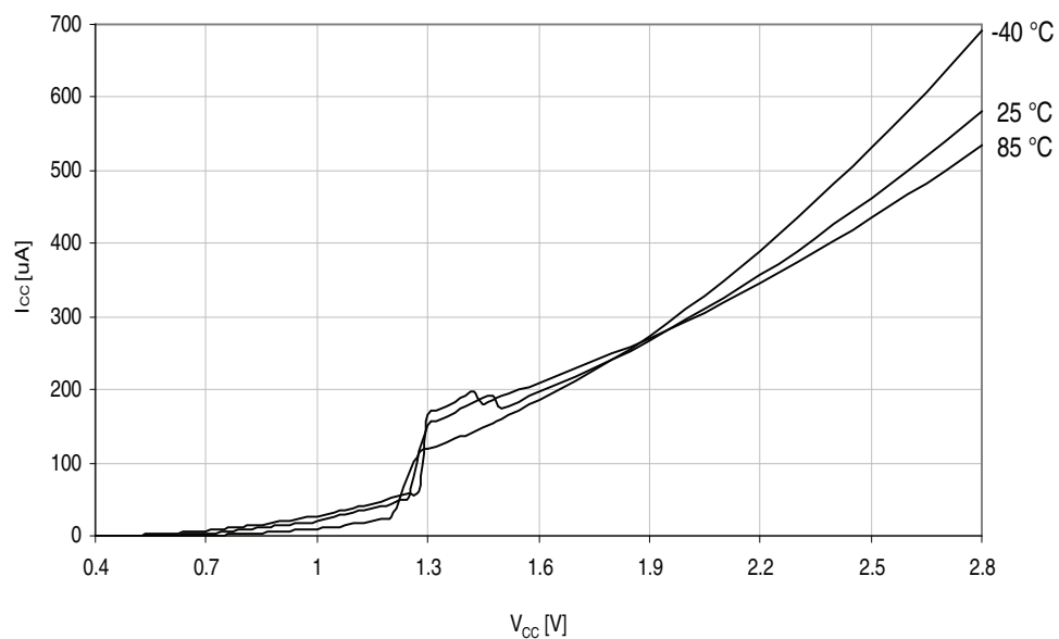
Figure 37-321. Power-on reset current consumption vs. V_{CC} .
