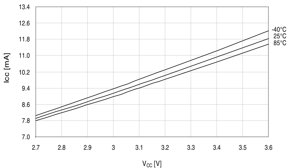
Figure 37-260. Active mode supply current vs. V_{CC} .
