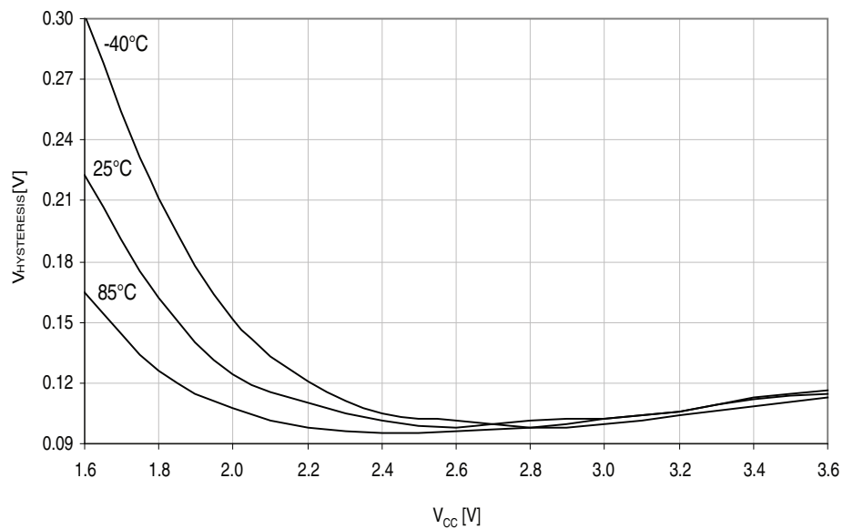
Figure 37-120. I/O pin input hysteresis vs. V_{CC} .
