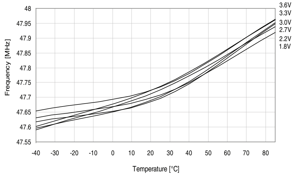
Figure 37-250.48MHz internal oscillator frequency vs. temperature. DPLL enabled, from the 32.768kHz internal oscillator.
