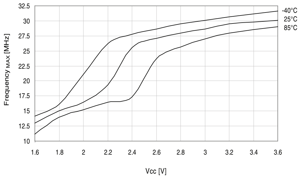
Figure 37-336.Maximum PDI frequency vs. V_{CC} .
