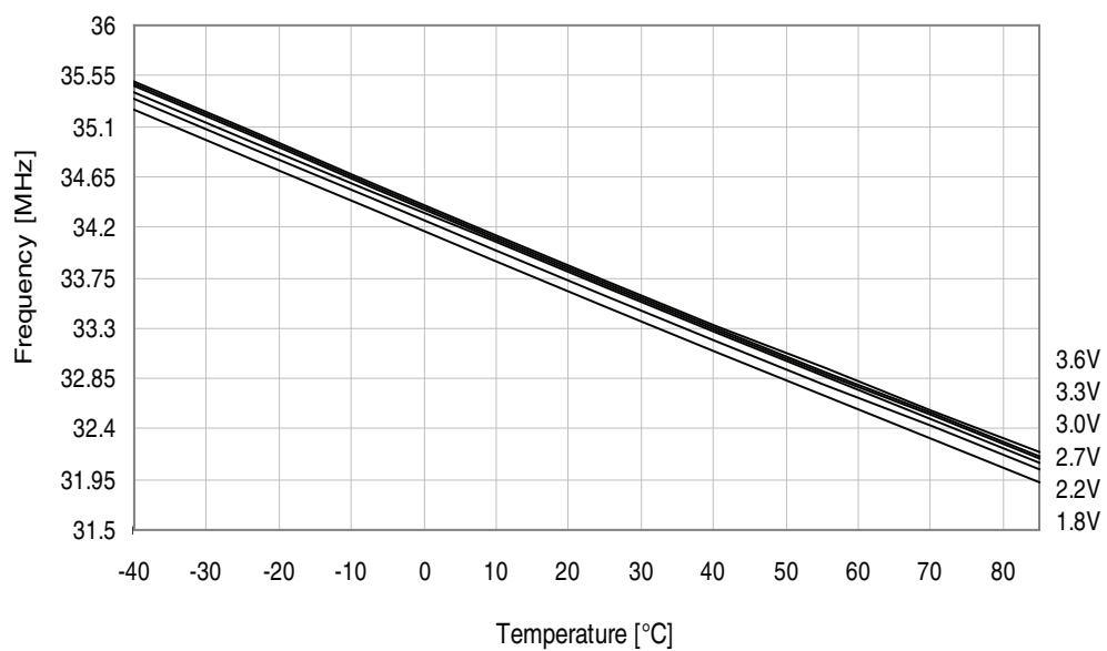
Figure 37-246. 32MHz internal oscillator frequency vs. temperature.
