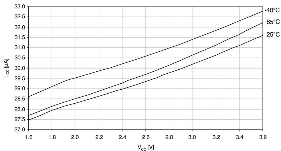
Figure 37-10. Idle mode supply current vs. V_{CC} .
