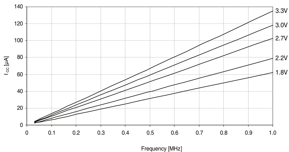
Figure 37-93. Idle mode supply current vs. frequency.
