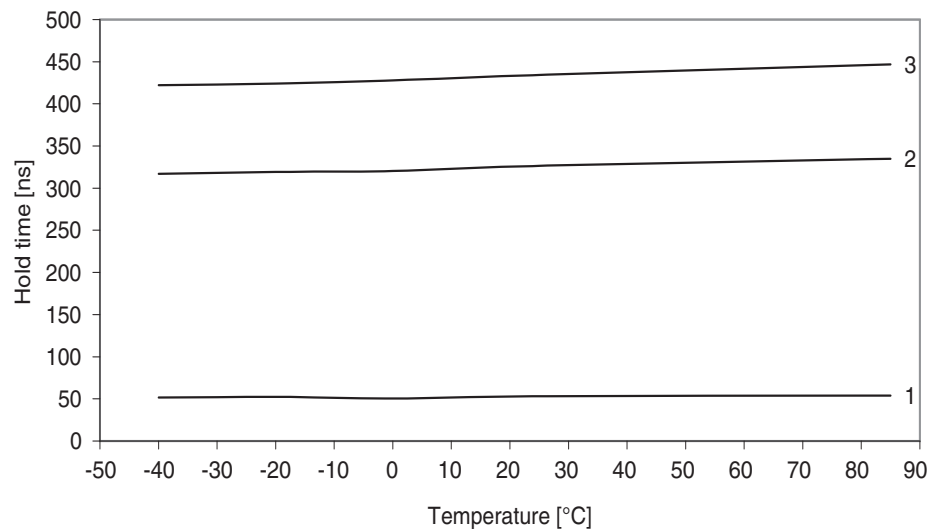
Figure 37-334.SDA hold time vs. temperature.
