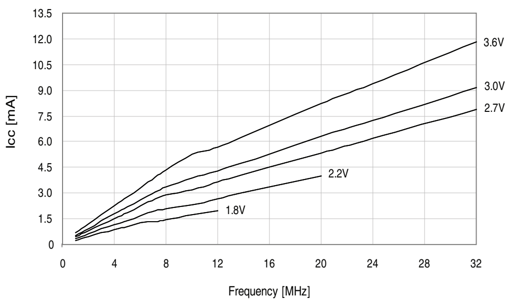
Figure 37-255.Active supply current vs. frequency.
