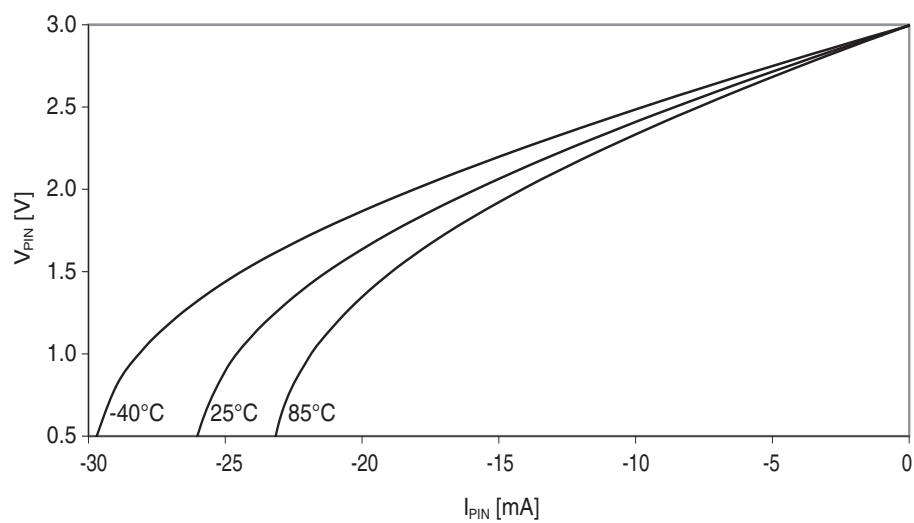
Figure 37-110. I/O pin output voltage vs. source current.
