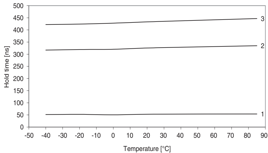
Figure 37-251.SDA hold time vs. temperature.
