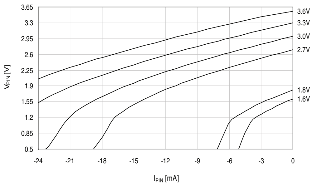
Figure 37-197. I/O pin output voltage vs. source current.
