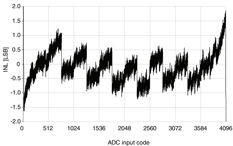
Figure 37-208. INL error vs. input code
