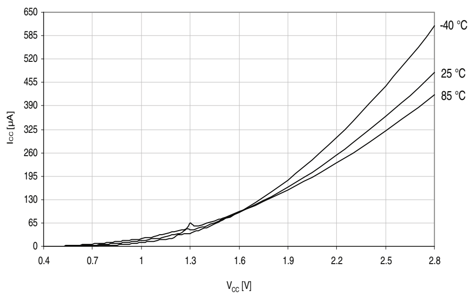
Figure 37-239. Power-on reset current consumption vs. V_{CC} . BOD level = 3.0V, enabled in sampled mode.
