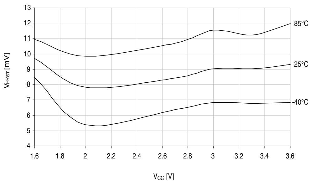
Figure 37-222.Analog comparator hysteresis vs. V_{CC} .
