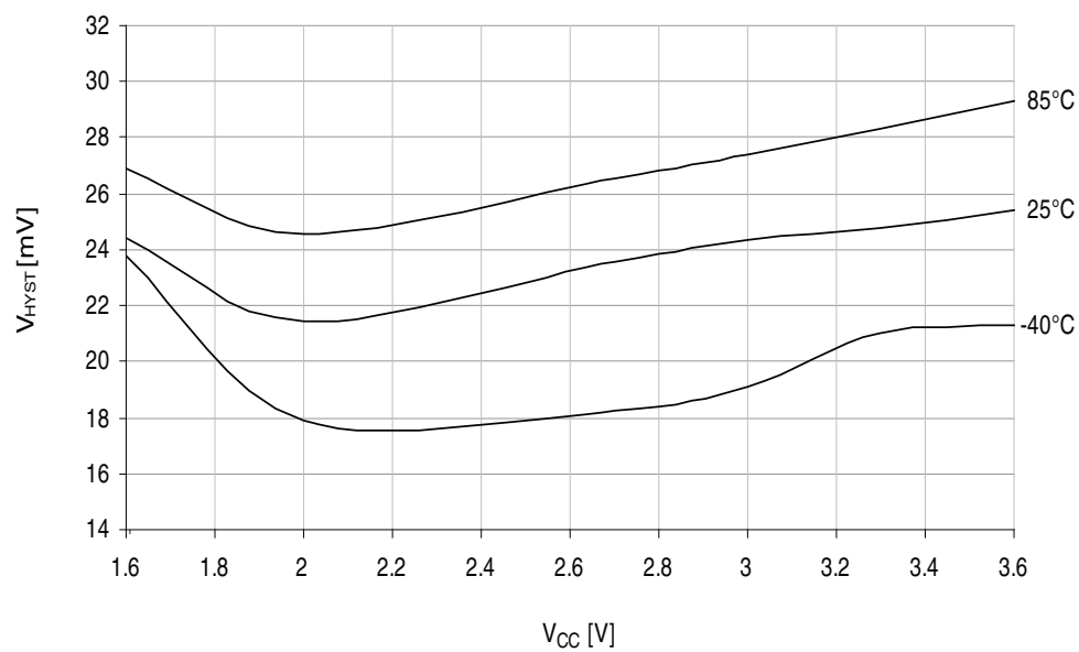
Figure 37-224. Analog comparator hysteresis vs. V_{CC} . High-speed mode, large hysteresis.
