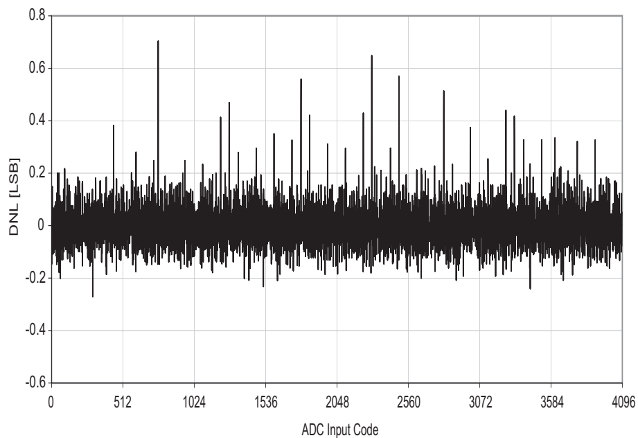
Figure 37-294.DNL error vs. input code.
