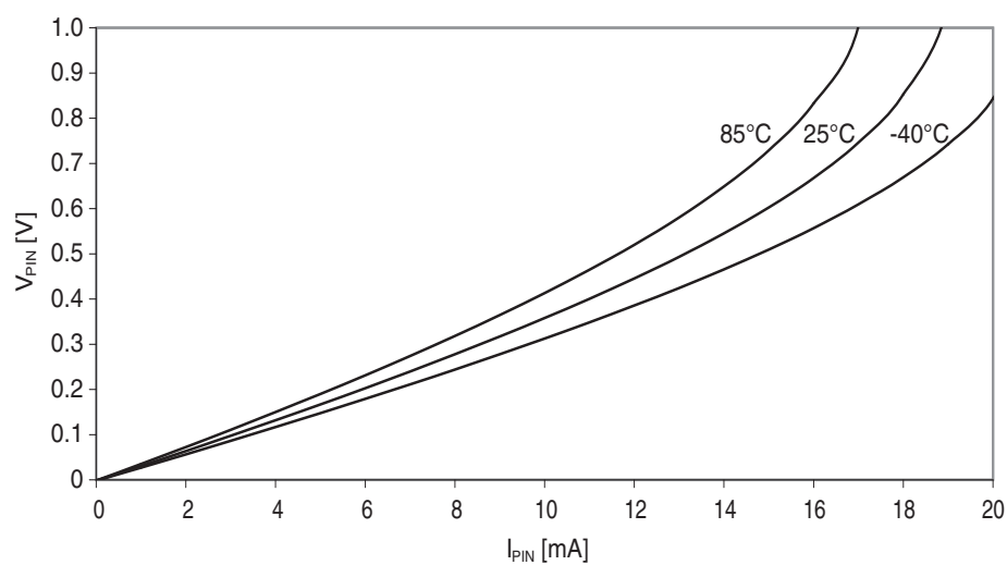
Figure 37-113. I/O pin output voltage vs. sink current.
