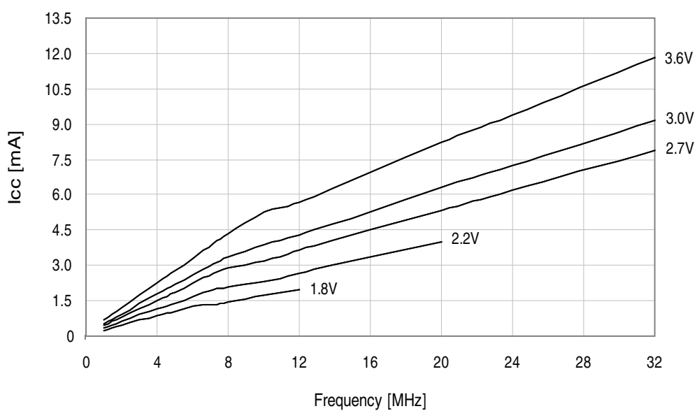
Figure 37-172.Active supply current vs. frequency.
