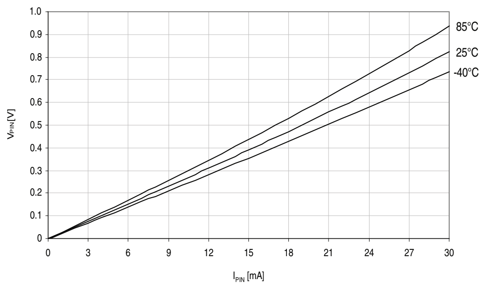
Figure 37-115. I/O pin output voltage vs. sink current.
