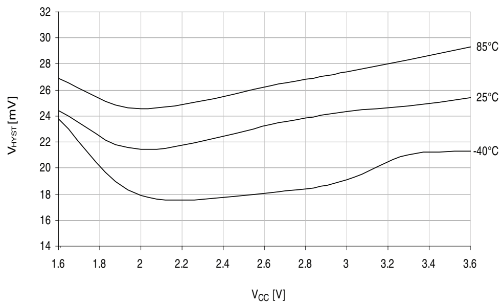
Figure 37-307. Analog comparator hysteresis vs. V_{CC} . High-speed mode, large hysteresis.
