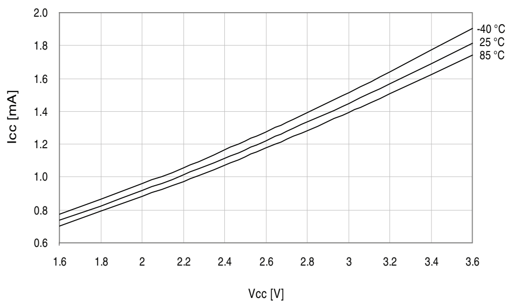
Figure 37-267. Idle mode current vs. V_{CC} .
