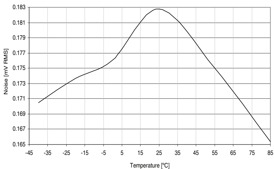
Figure 37-304.DAC noise vs. temperature.
