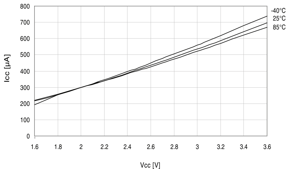
Figure 37-257. Active mode supply current vs. V_{CC} .
