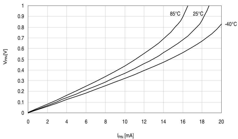
Figure 37-198. I/O pin output voltage vs. sink current.
