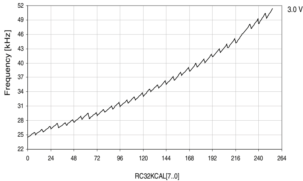
Figure 37-325.32.768kHz internal oscillator frequency vs. calibration value.
