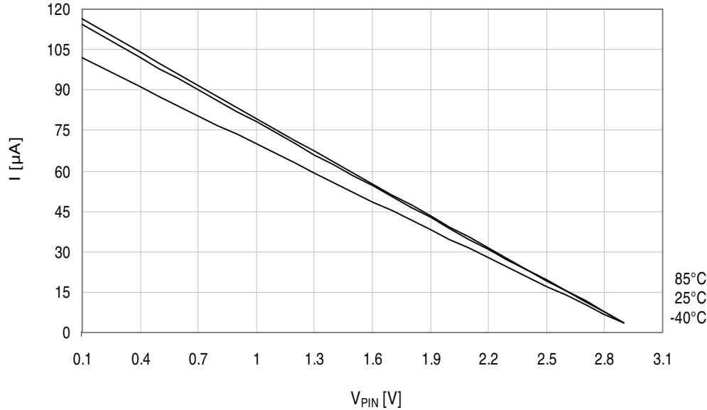
Figure 37-275. I/O pin pull-up resistor current vs. input voltage. V_{CC} = 3.0V .
