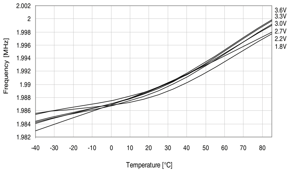
Figure 37-244.2MHz internal oscillator frequency vs. temperature. DPLL enabled, from the 32.768kHz internal oscillator .
