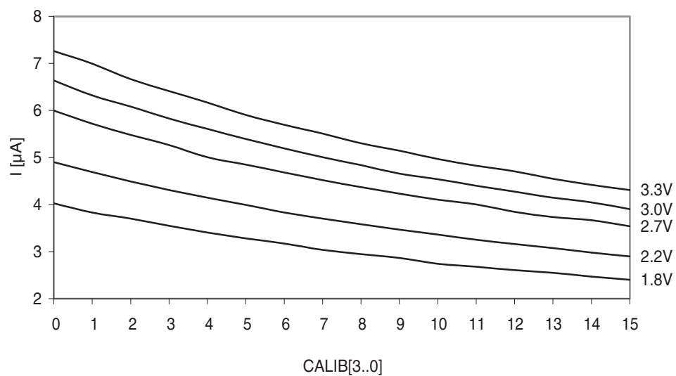
Figure 37-141. Analog comparator current source vs. calibration value.
