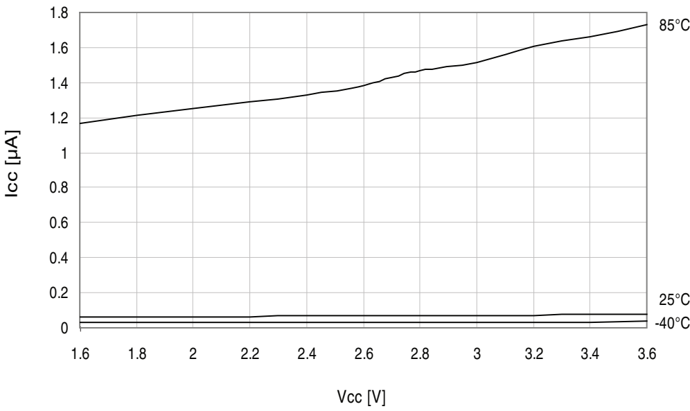
Figure 37-269. Power-down mode supply current vs. V_{CC} . All functions disabled.
