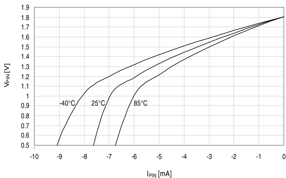
Figure 37-277. I/O pin output voltage vs. source current.
