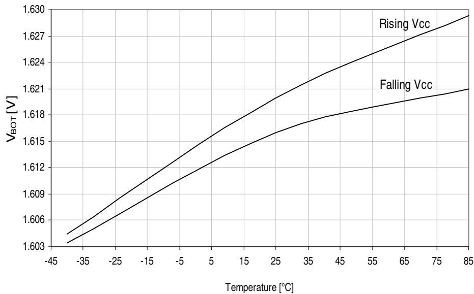
Figure 37-145.BOD thresholds vs. temperature. BOD level = 1.6V.
