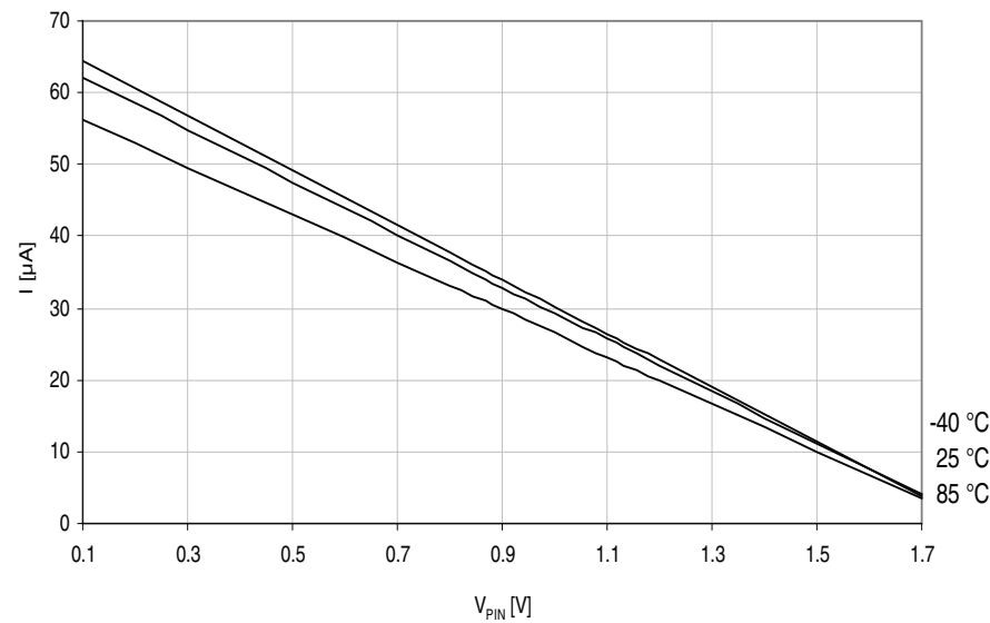
Figure 37-106. I/O pin pull-up resistor current vs. input voltage. V_{CC} = 1.8V .
