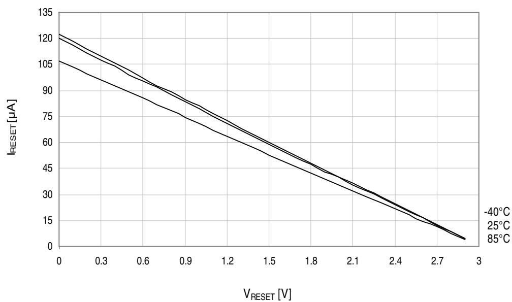
Figure 37-234. Reset pin pull-up resistor current vs. reset pin voltage.
