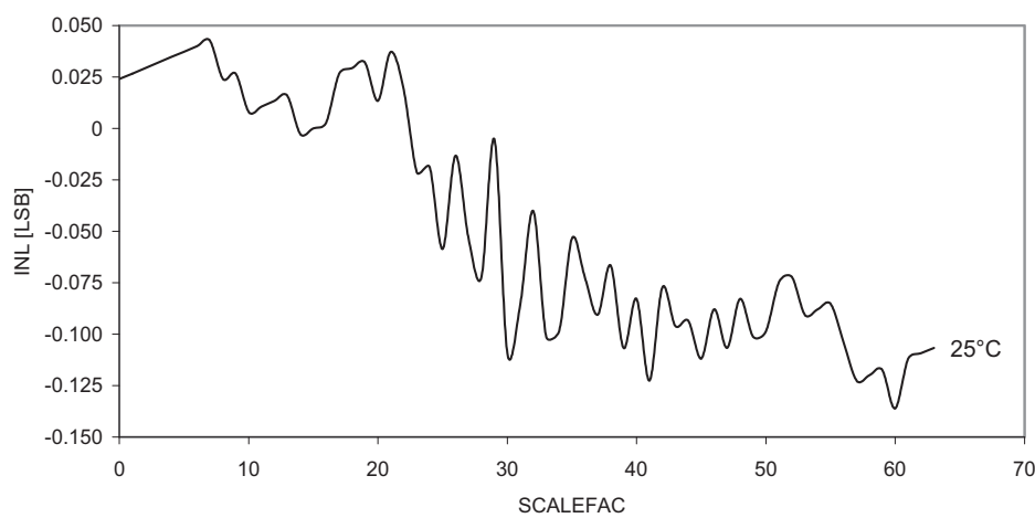
Figure 37-311. Voltage scaler INL vs. SCALEFAC.
