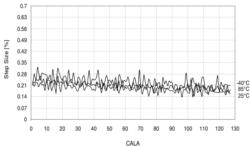
Figure 37-248. 32MHz internal oscillator CALA calibration step size.
