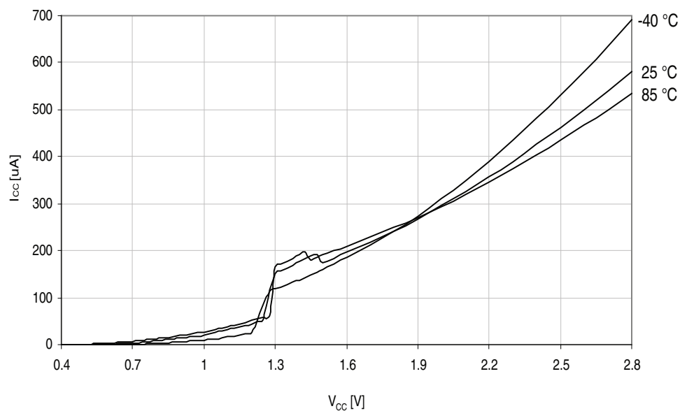
Figure 37-238. Power-on reset current consumption vs. V_{CC} .
