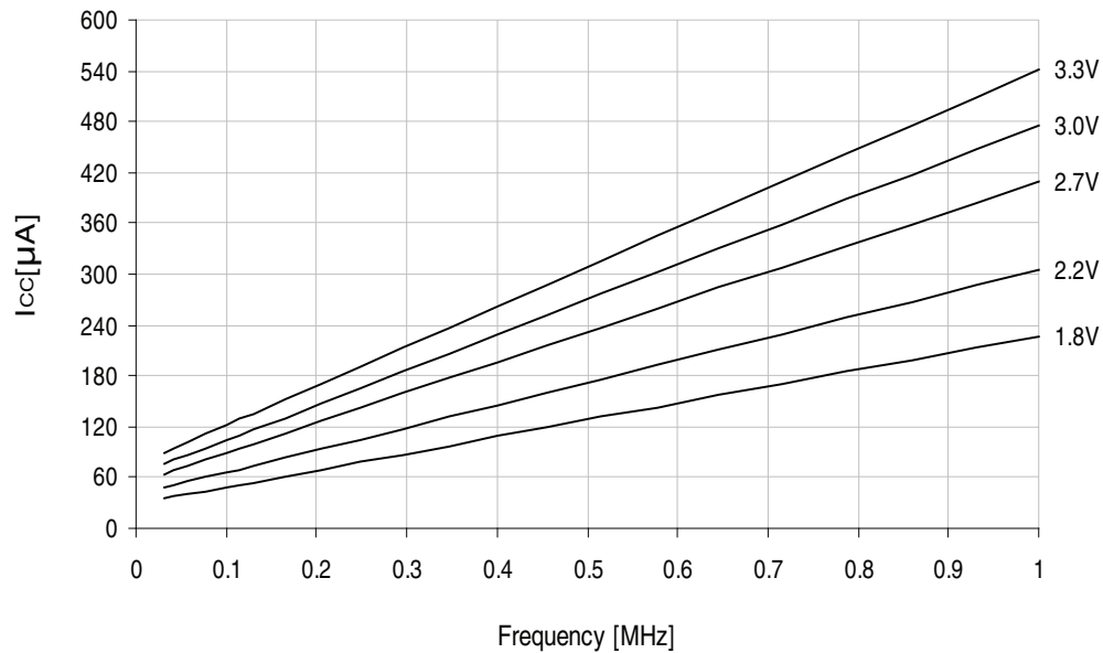
Figure 37-87. Active supply current vs. frequency.
