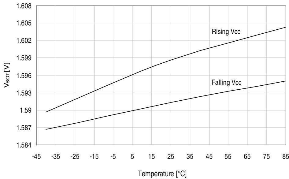
Figure 37-313.BOD thresholds vs. temperature.
