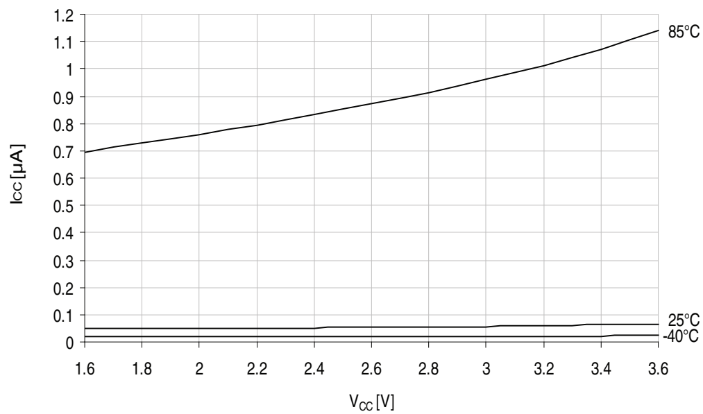
Figure 37-16. Power-down mode supply current vs. V_{CC} .
