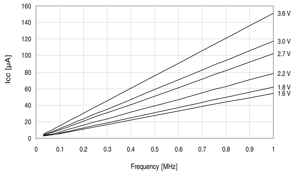
Figure 37-178.Idle mode supply current vs. frequency.
