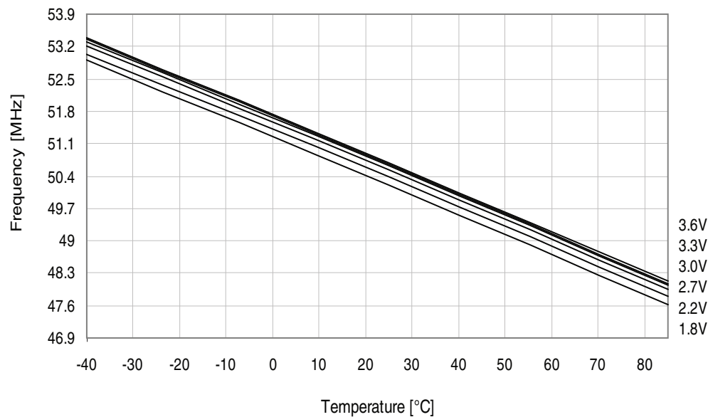
Figure 37-333.48MHz internal oscillator frequency vs. temperature. DPLL enabled, from the 32.768kHz internal oscillator.
