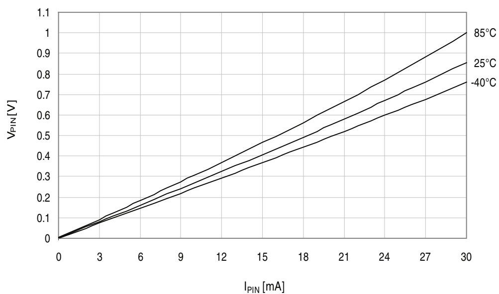
Figure 37-200. I/O pin output voltage vs. sink current.
