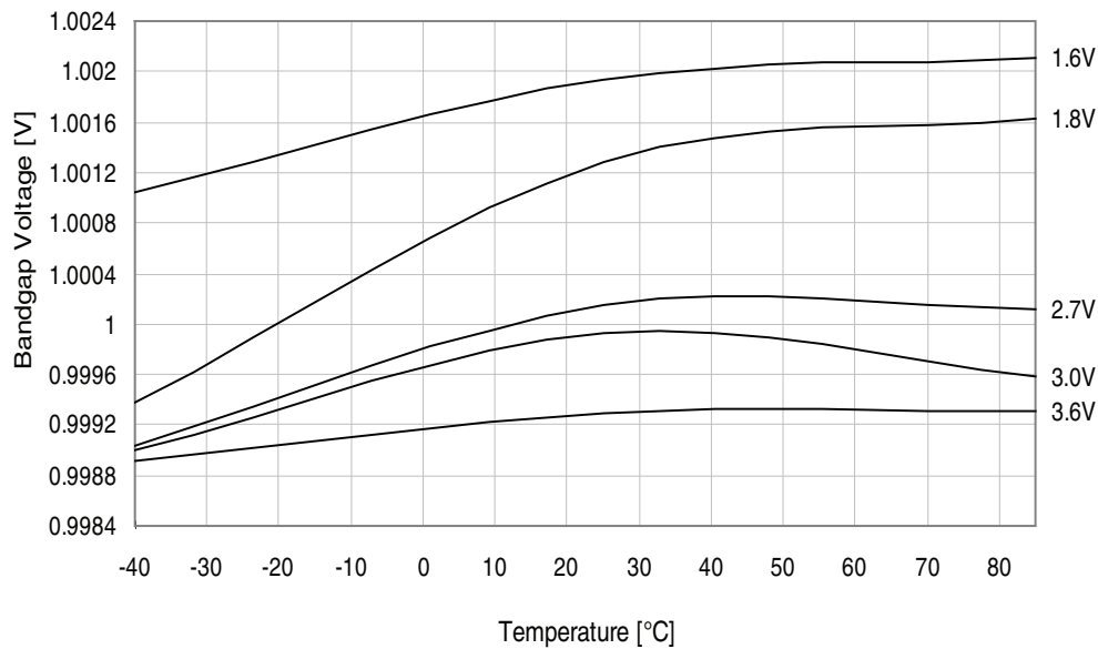
Figure 37-312.ADC/DAC Internal 1.0V reference vs. temperature.
