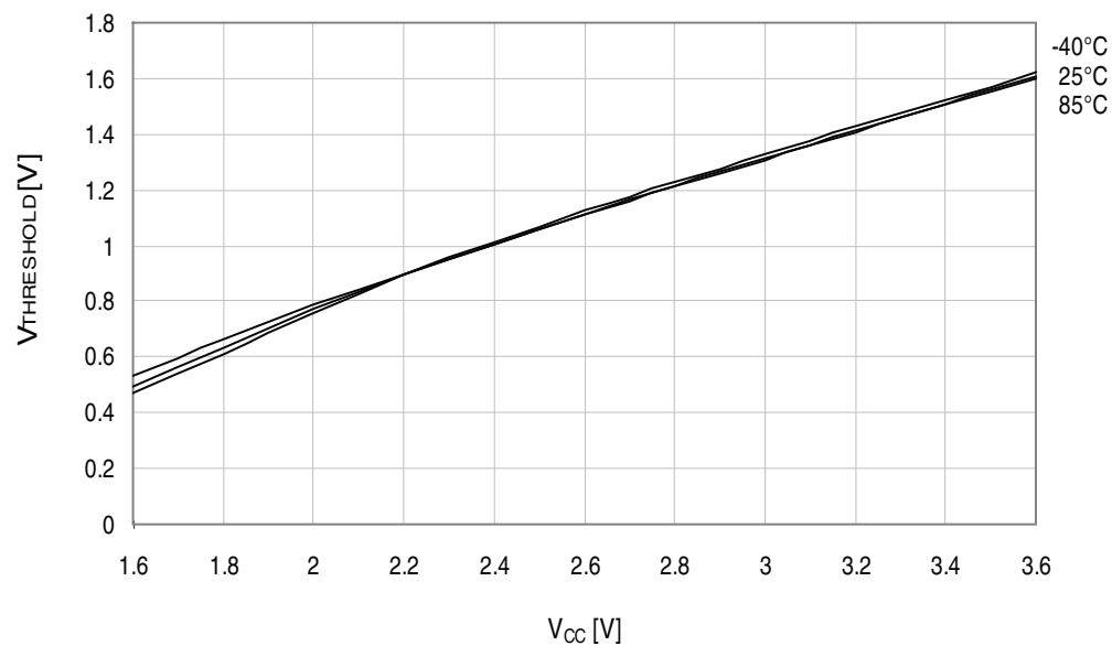
Figure 37-319. Reset pin input threshold voltage vs. V_{CC} .
