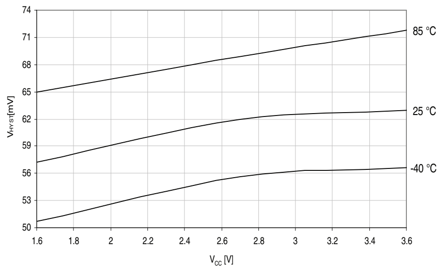
Figure 37-140. Analog comparator hysteresis vs. V_{CC} .
