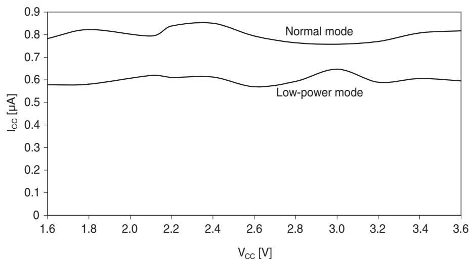
Figure 37-271. Power-save mode supply current vs. V_{CC} . Real Time Counter enabled and running from 1.024kHz output of 32.768kHz TOSC.
