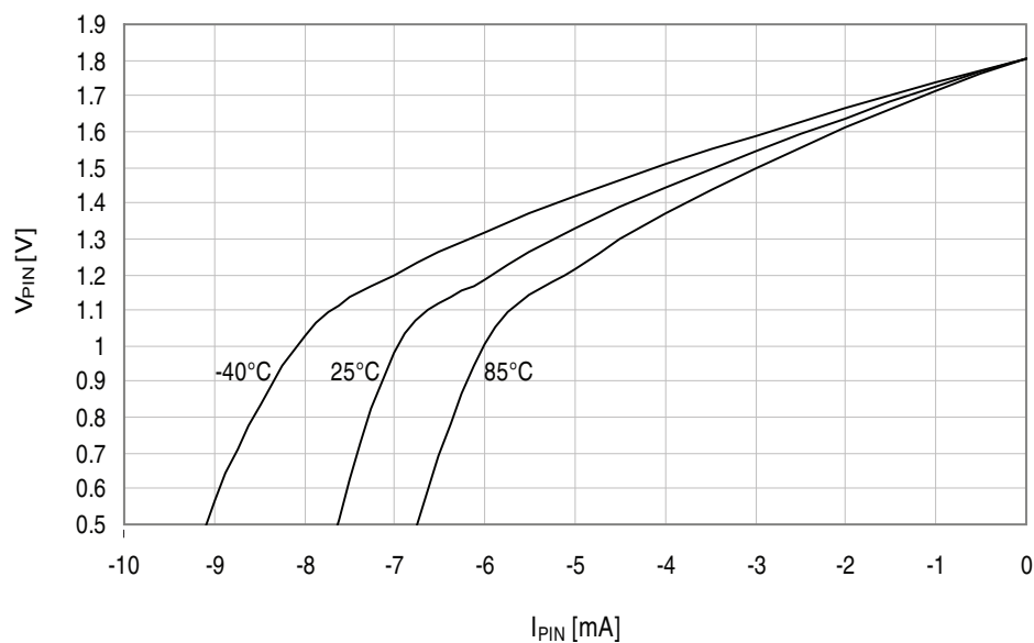
Figure 37-194. I/O pin output voltage vs. source current.
