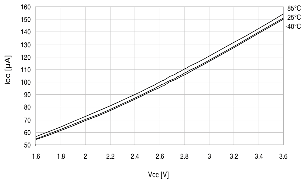
Figure 37-182. Idle mode supply current vs. V_{CC} .
