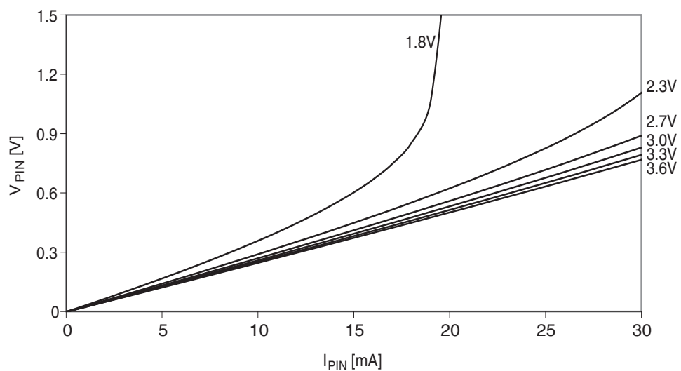
Figure 37-116. I/O pin output voltage vs. sink current.
