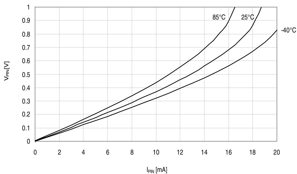
Figure 37-281. I/O pin output voltage vs. sink current.
