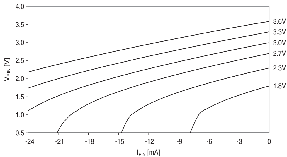
Figure 37-112. I/O pin output voltage vs. source current.
