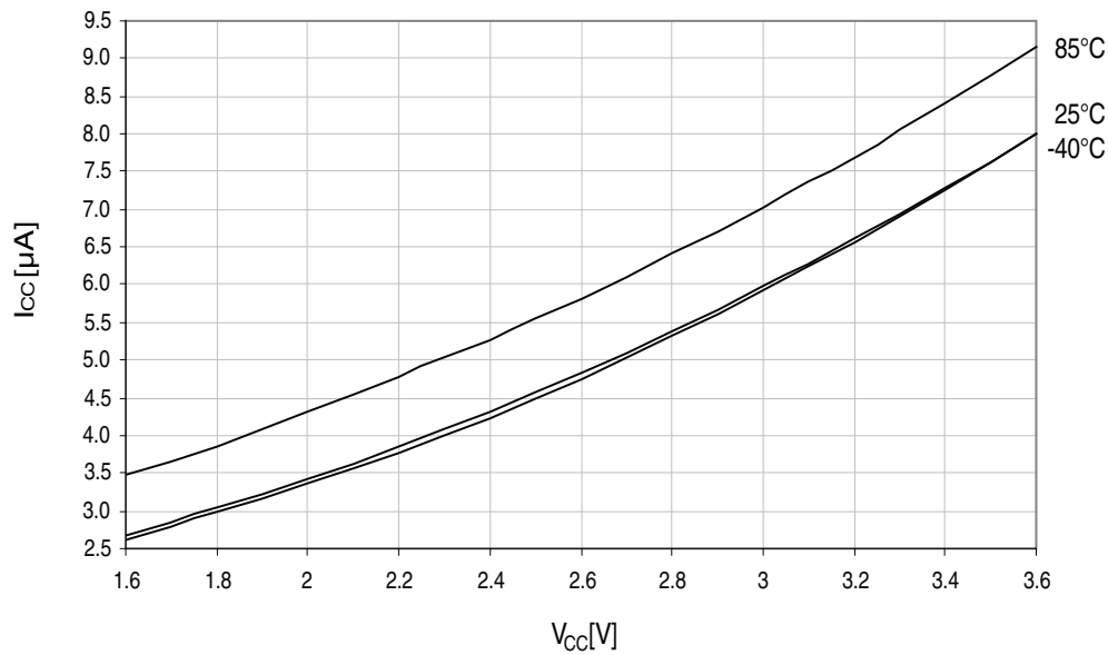
Figure 37-273. Standby supply current vs. V_{CC} .
