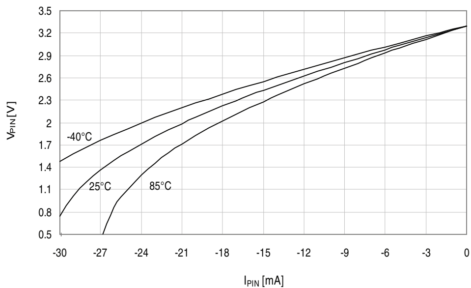
Figure 37-196. I/O pin output voltage vs. source current.
