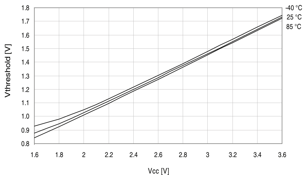
Figure 37-286. I/O pin input threshold voltage vs. V_{CC} .
