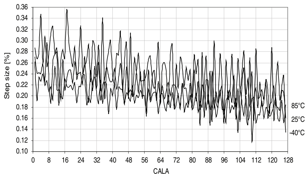
Figure 37-78. 32MHz internal oscillator CALA calibration step size. V_{CC} = 3.0V .
