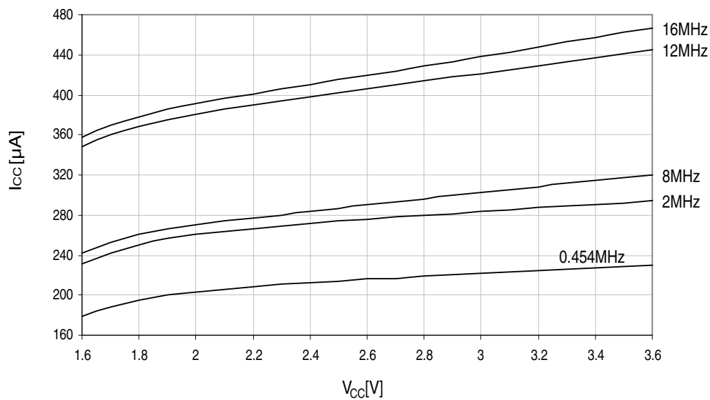
Figure 37-273. Standby supply current vs. V_{CC} .
