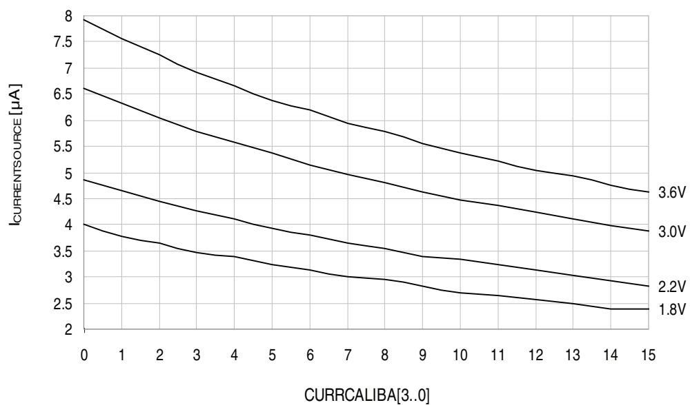
Figure 37-309. Analog comparator current source vs. calibration value. Temperature = 25°C.
