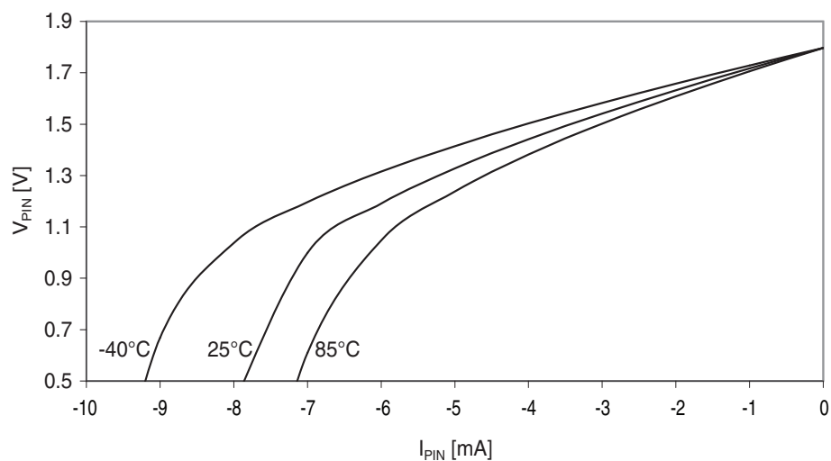
Figure 37-109. I/O pin output voltage vs. source current.
