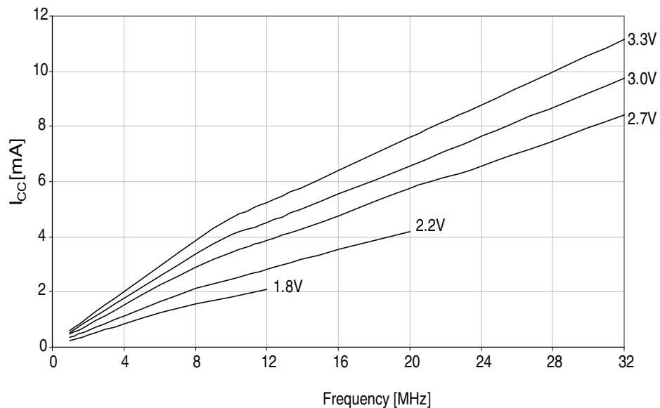
Figure 37-87. Active supply current vs. frequency.
