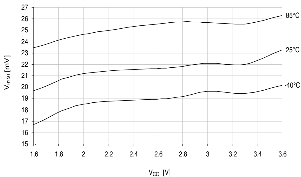
Figure 37-224. Analog comparator hysteresis vs. V_{CC} . High-speed mode, large hysteresis.
