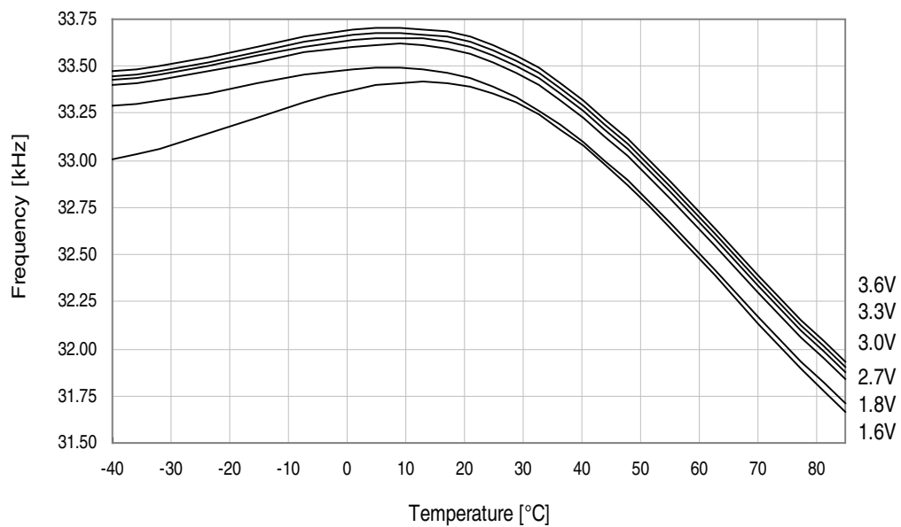
Figure 37-323. Ultra Low-Power internal oscillator frequency vs. temperature.
