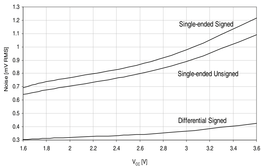
Figure 37-301. Noise vs. V_{CC} .
