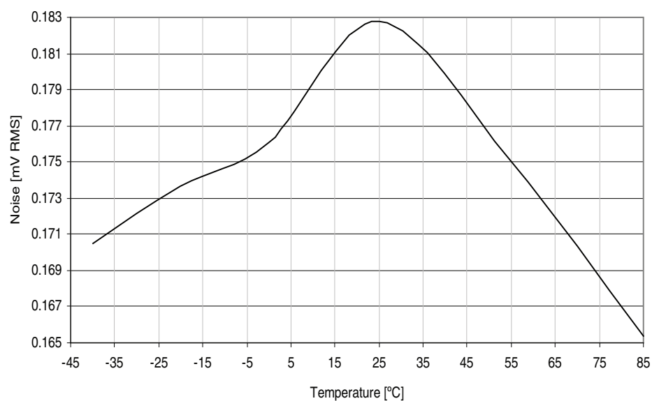
Figure 37-221.DAC noise vs. temperature.
