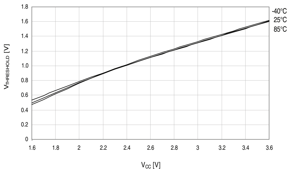
Figure 37-237. Reset pin input threshold voltage vs. V_{CC} .
