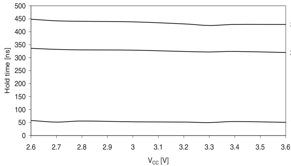
Figure 37-335.SDA hold time vs. supply voltage.
