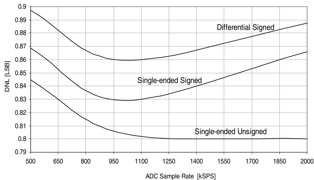
Figure 37-210.DNL error vs. sample rate. T = 25^{\circ}\text{C} , V_{CC} = 3.6\text{V} , V_{REF} = 3.0\text{V} external.
