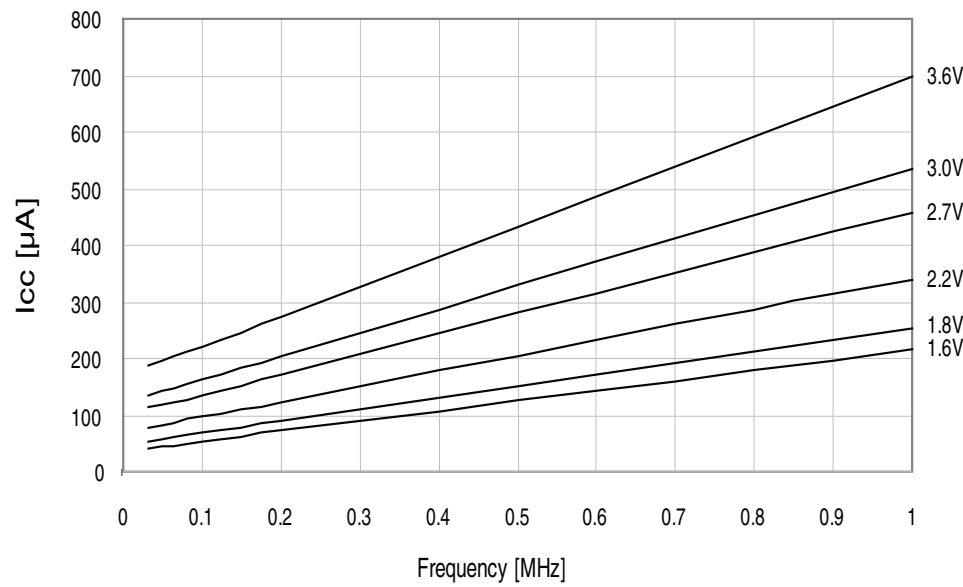
Figure 37-172.Active supply current vs. frequency.
