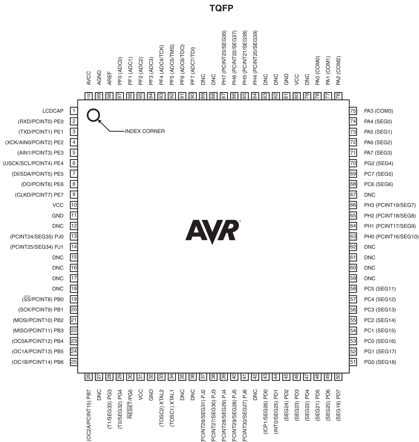
Figure 1-2. Pinout ATmega3290A/ATmega3290PA/ATmega6490A/ATmega6490P
