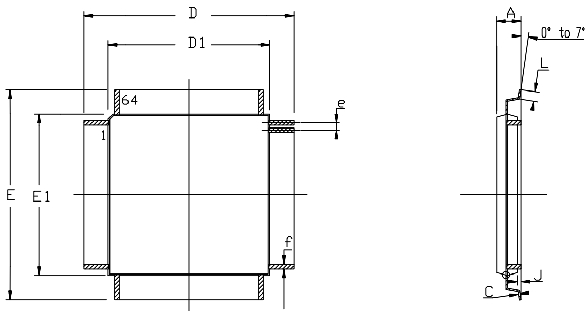
Figure 12-3. 64-lead LQFP Package Mechanical Drawing
