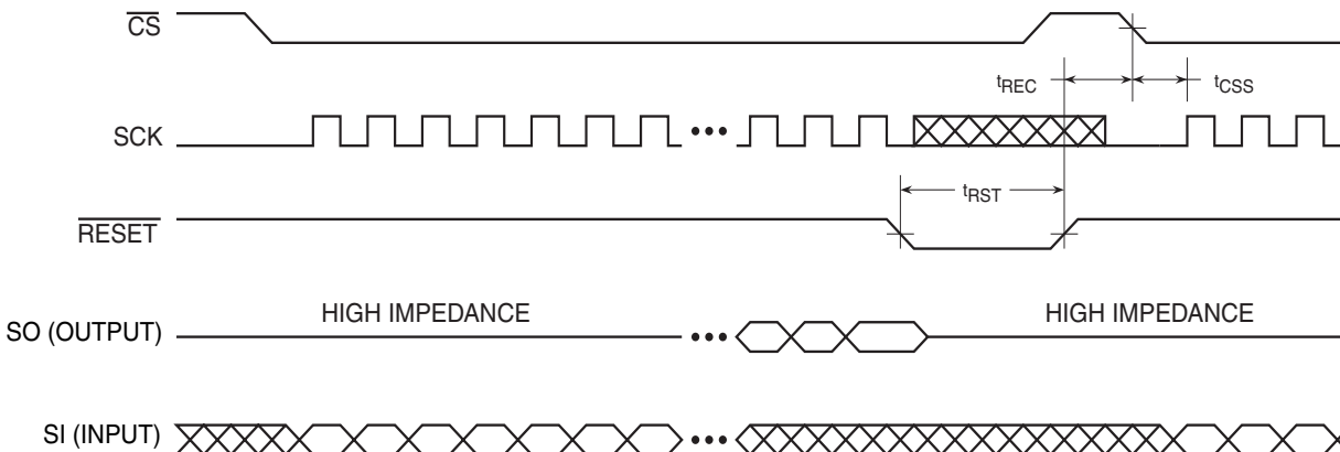
Figure 17-6. Reset Timing
