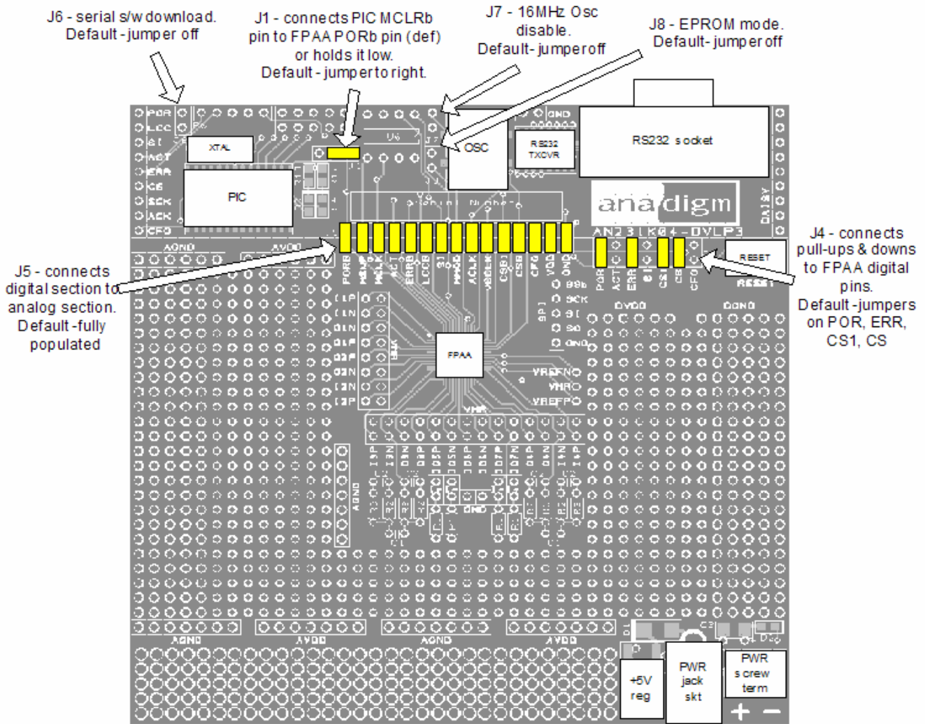
Figure 4: Positions of Jumpers and Default Settings
