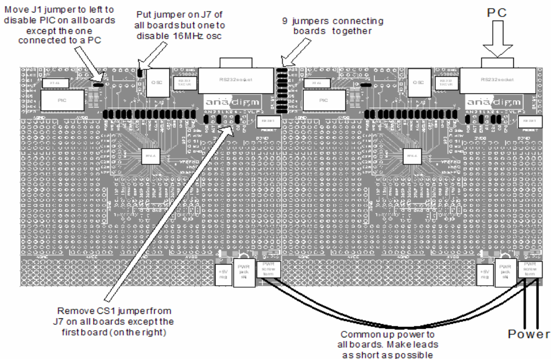
Figure 3: Positions of Jumpers and Default Settings
