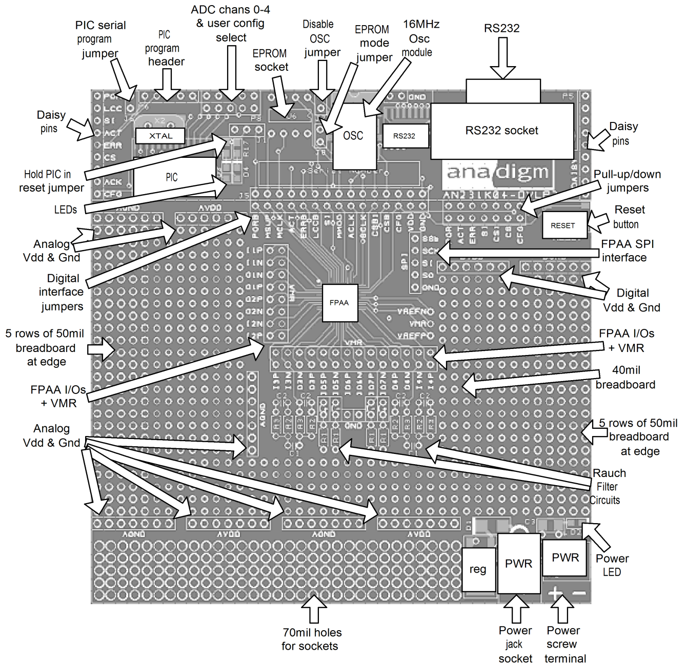
Figure 2: Top-level layout of the AnadigmApex development board
