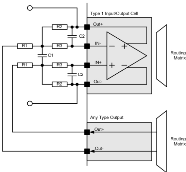
Type 1 I/O Configured as a Smoothing Filter for an Output Cell
