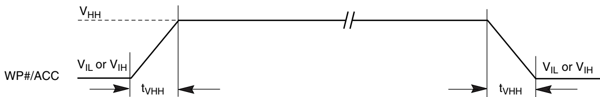
Figure I8. Accelerated Program Timing Diagram
