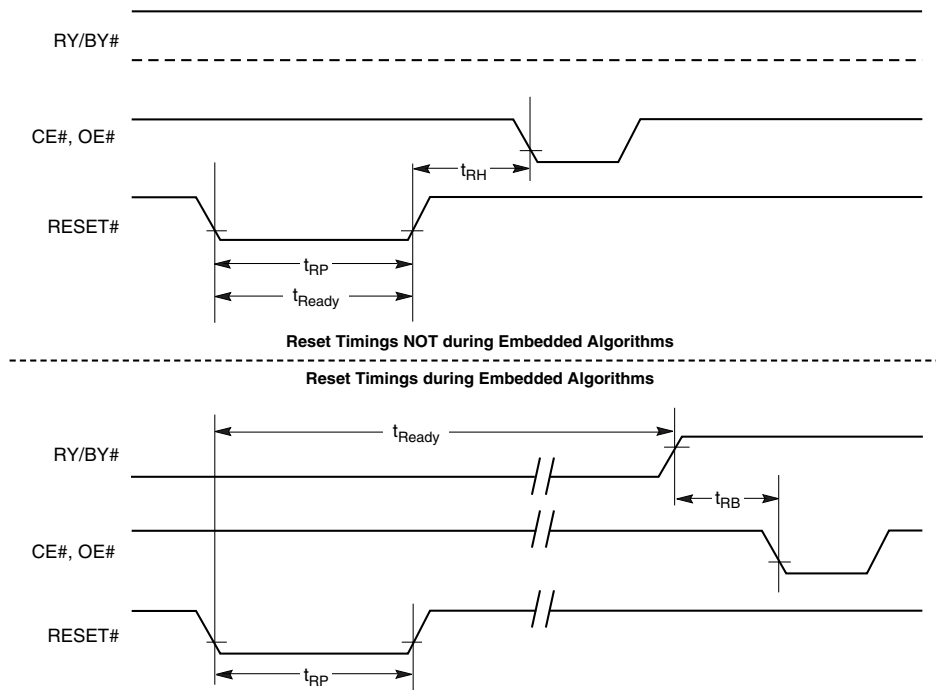
Figure I4. Reset Timings
