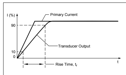
Step Response
