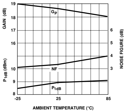
Figure 5. Power Gain, Noise Figure, and P_{1dB} vs. Temperature at 1 GHz and I_D = 29 mA.
