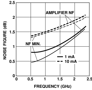
Figure 2. AT-31011 and AT-31033 Minimum Noise Figure and Amplifier \text{NF}^{(1)} vs. Frequency and Current at V_{\text{CE}} = 2.7\text{ V} .
