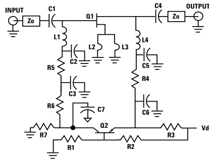
Figure 1. Typical ATF-54143 LNA with Passive Biasing.
