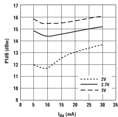
Figure 20. P1dB vs. I_{dq} and V_{ds} at 900 MHz. [1,2]
