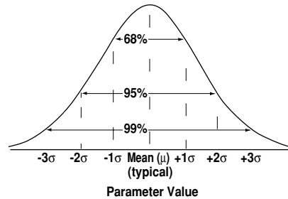
Figure 19. Normal Distribution.
