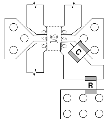
Figure 21. RF Layout.
