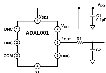
Figure 1. EVAL-ADXL001 Schematic
