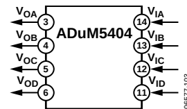
Figure 5. ADuM5404
