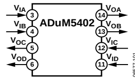
Figure 3. ADuM5402
