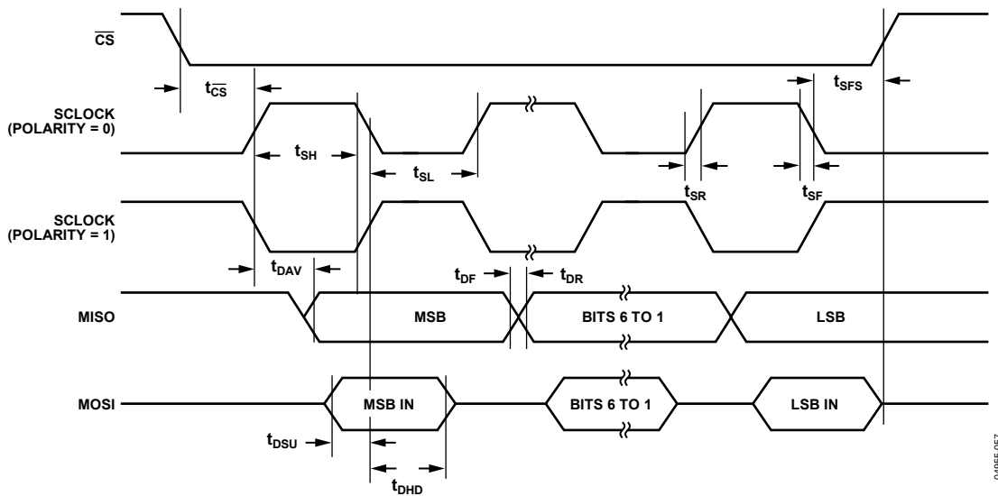
Figure 8. SPI Slave Mode Timing (Phase Mode = 1)
