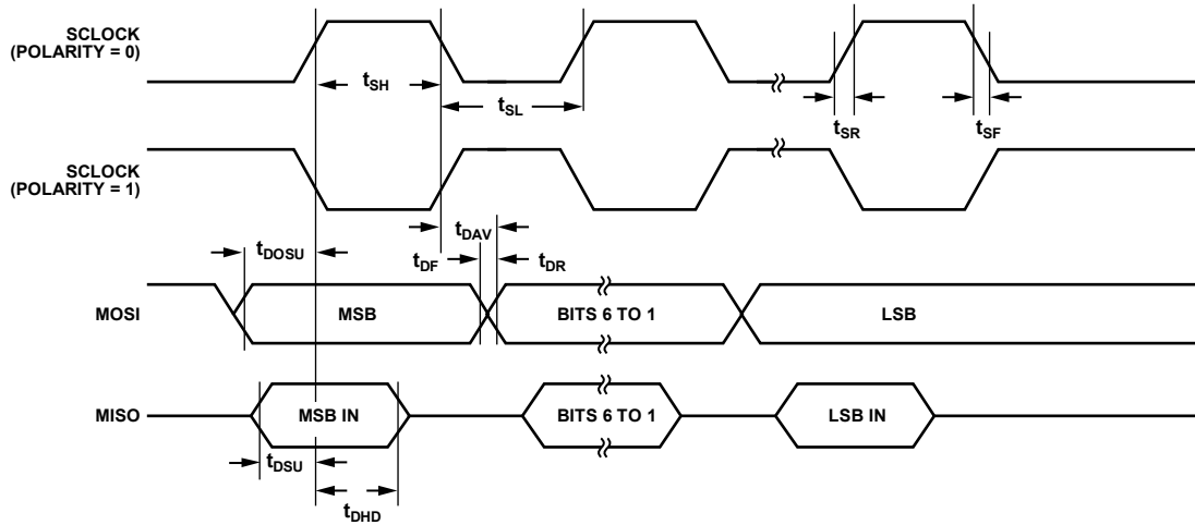
Figure 7. SPI Master Mode Timing (Phase Mode = 0)
