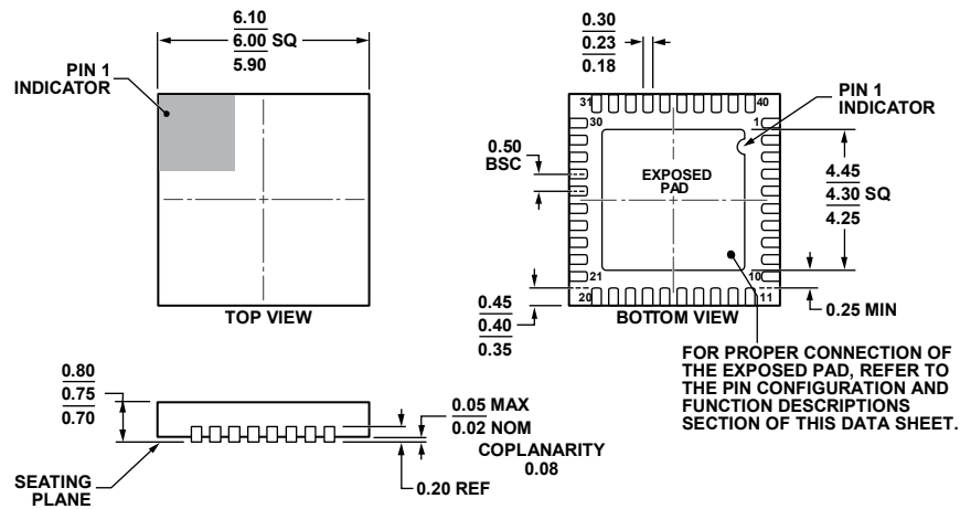
Figure 84. 40-Lead Lead Frame Chip Scale Package [LFCSP_VQ] 6 mm × 6 mm Body, Very Thin Quad (CP-40-1) Dimensions shown in millimeters
