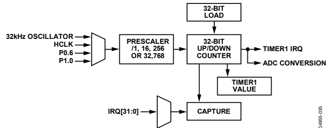
Figure 66. Timer1 Block Diagram
