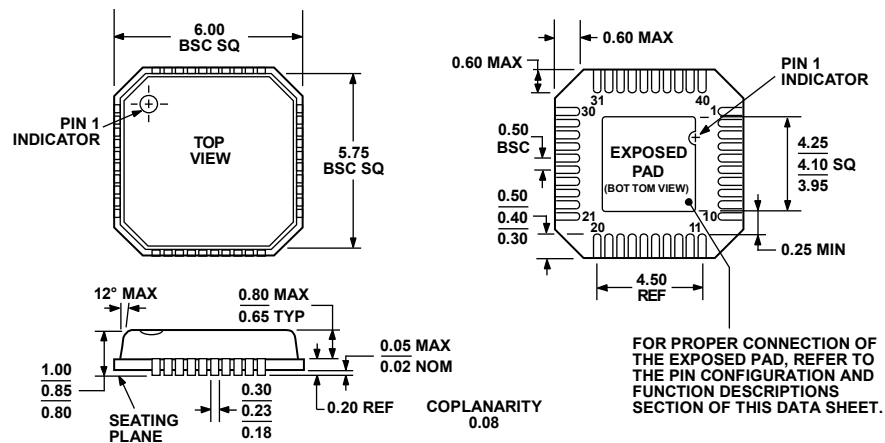
Figure 84. 40-Lead Lead Frame Chip Scale Package [LFCSP_VQ] 6 mm × 6 mm Body, Very Thin Quad (CP-40-1) Dimensions shown in millimeters
