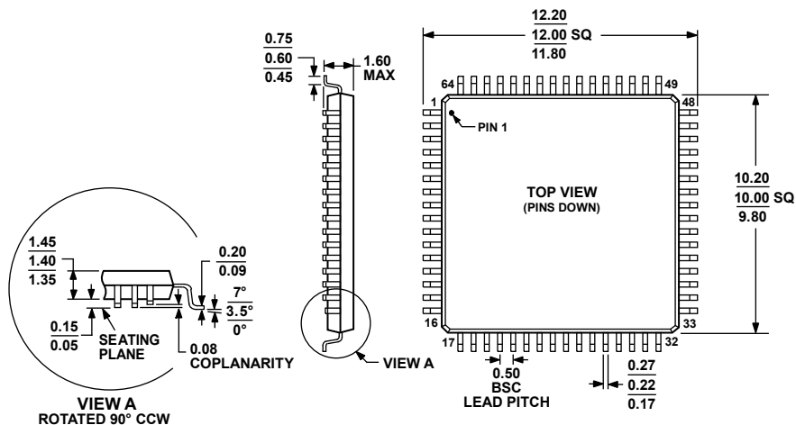
Figure 87. 64-Lead Low Profile Quad Flat Package [LQFP] (ST-64-2) Dimensions shown in millimeters
