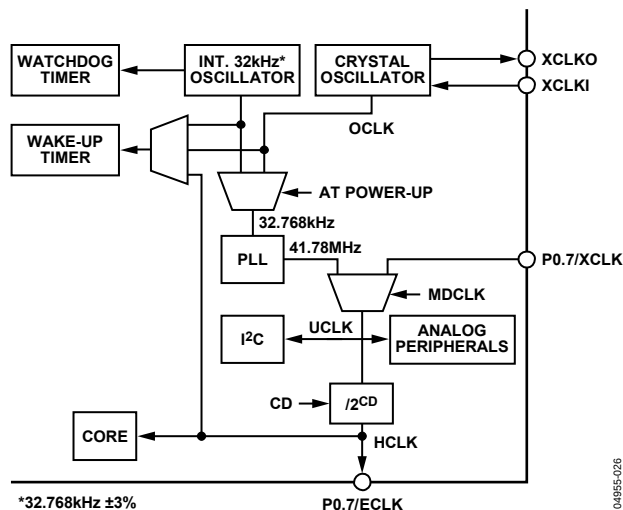
Figure 57. Clocking System
